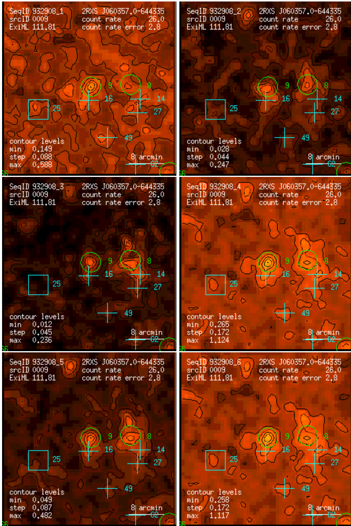
Figure 9: RASS 932908: detection 0009: band rate images, Gaussian filter: (1) PSPC channels 11 – 41, (2) 52 – 90, (3) 91 – 201, (4) 11 – 235, (5) 52 – 201, (6) 11 – 201. Broad band rates in counts/ks. Band rate contour levels in counts/ks/arcmin 2 .
