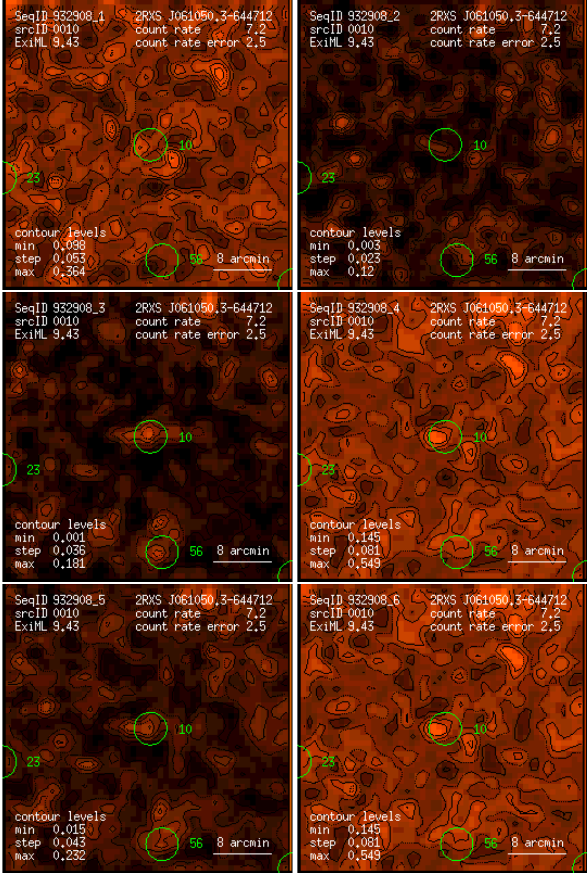
Figure 10: RASS 932908: detection 0010: band rate images, Gaussian filter: (1) PSPC channels 11 – 41, (2) 52 – 90, (3) 91 – 201, (4) 11 – 235, (5) 52 – 201, (6) 11 – 201. Broad band rates in counts/ks. Band rate contour levels in counts/ks/arcmin 2 .
