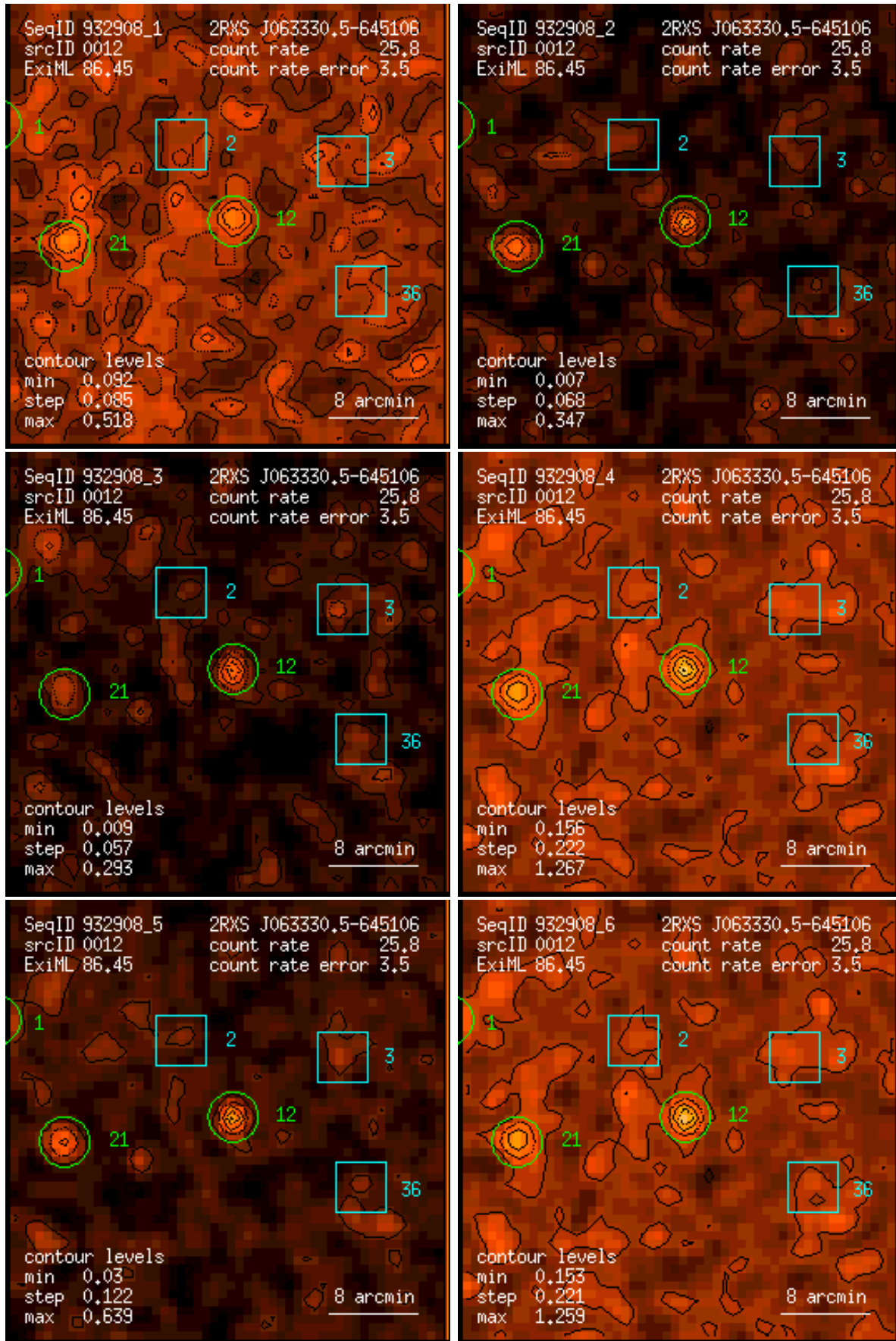
Figure 12: RASS 932908: detection 0012: band rate images, Gaussian filter: (1) PSPC channels 11 – 41, (2) 52 – 90, (3) 91 – 201, (4) 11 – 235, (5) 52 – 201, (6) 11 – 201. Broad band rates in counts/ks. Band rate contour levels in counts/ks/arcmin 2 .
