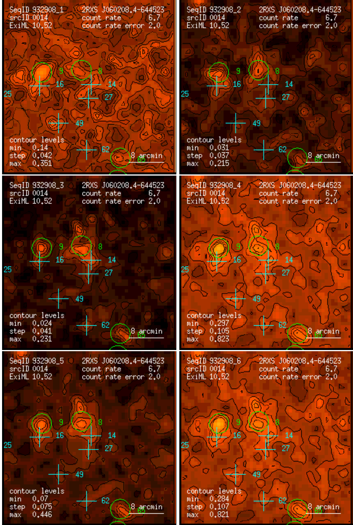
Figure 14: RASS 932908: detection 0014: band rate images, Gaussian filter: (1) PSPC channels 11 – 41, (2) 52 – 90, (3) 91 – 201, (4) 11 – 235, (5) 52 – 201, (6) 11 – 201. Broad band rates in counts/ks. Band rate contour levels in counts/ks/arcmin 2 .
