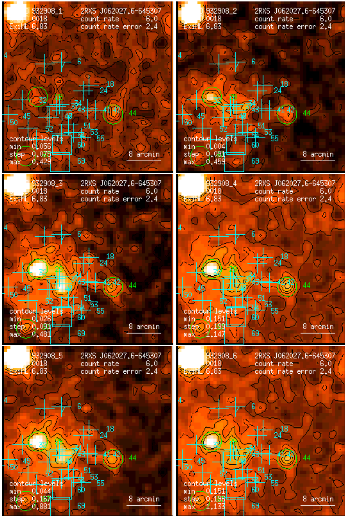
Figure 18: RASS 932908: detection 0018: band rate images, Gaussian filter: (1) PSPC channels 11 – 41, (2) 52 – 90, (3) 91 – 201, (4) 11 – 235, (5) 52 – 201, (6) 11 – 201. Broad band rates in counts/ks. Band rate contour levels in counts/ks/arcmin 2 .
