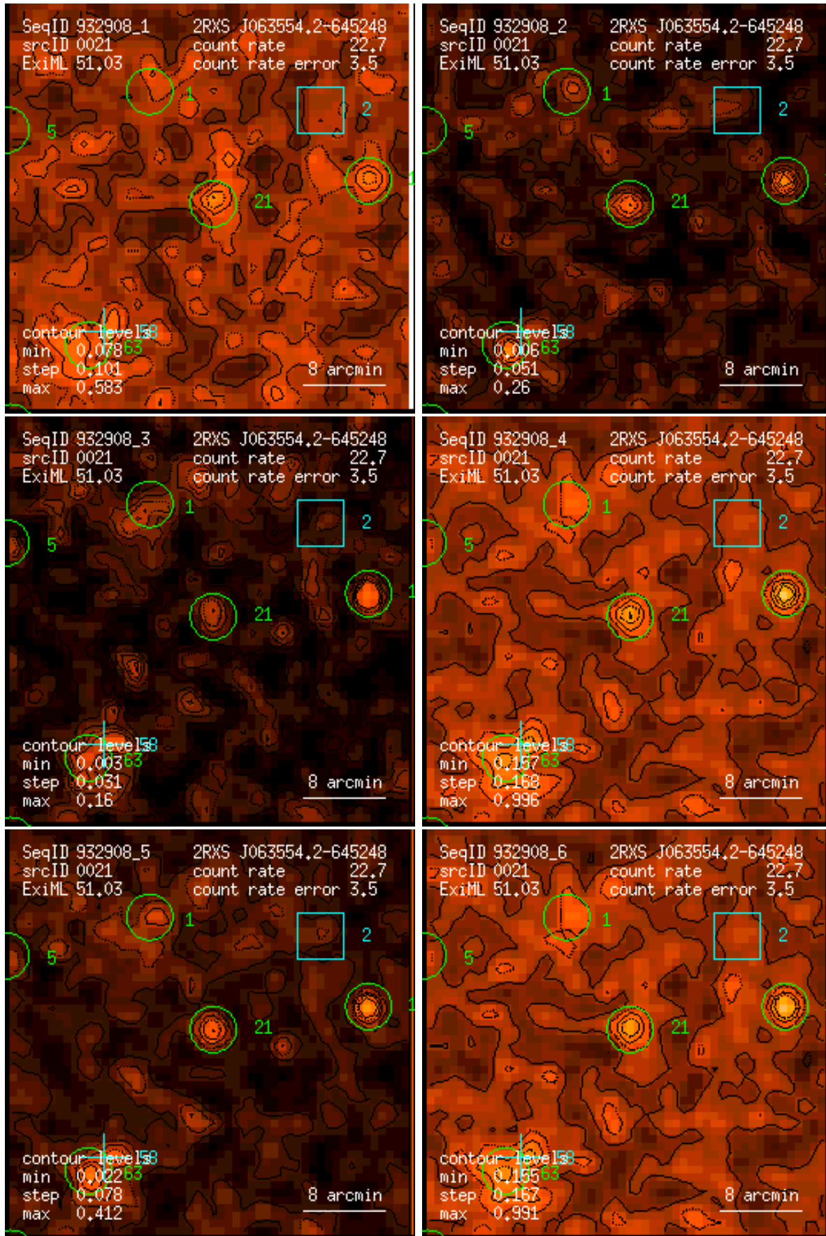
Figure 21: RASS 932908: detection 0021: band rate images, Gaussian filter: (1) PSPC channels 11 – 41, (2) 52 – 90, (3) 91 – 201, (4) 11 – 235, (5) 52 – 201, (6) 11 – 201. Broad band rates in counts/ks. Band rate contour levels in counts/ks/arcmin 2 .
