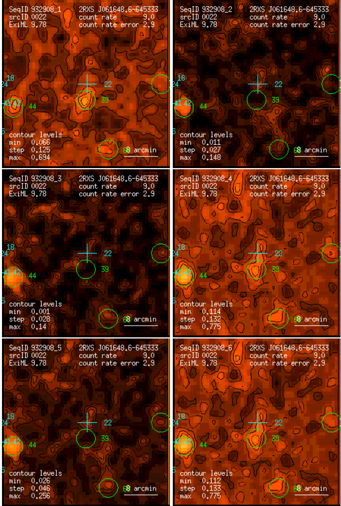
Figure 22: RASS 932908: detection 0022: band rate images, Gaussian filter: (1) PSPC channels 11 – 41, (2) 52 – 90, (3) 91 – 201, (4) 11 – 235, (5) 52 – 201, (6) 11 – 201. Broad band rates in counts/ks. Band rate contour levels in counts/ks/arcmin 2 .
