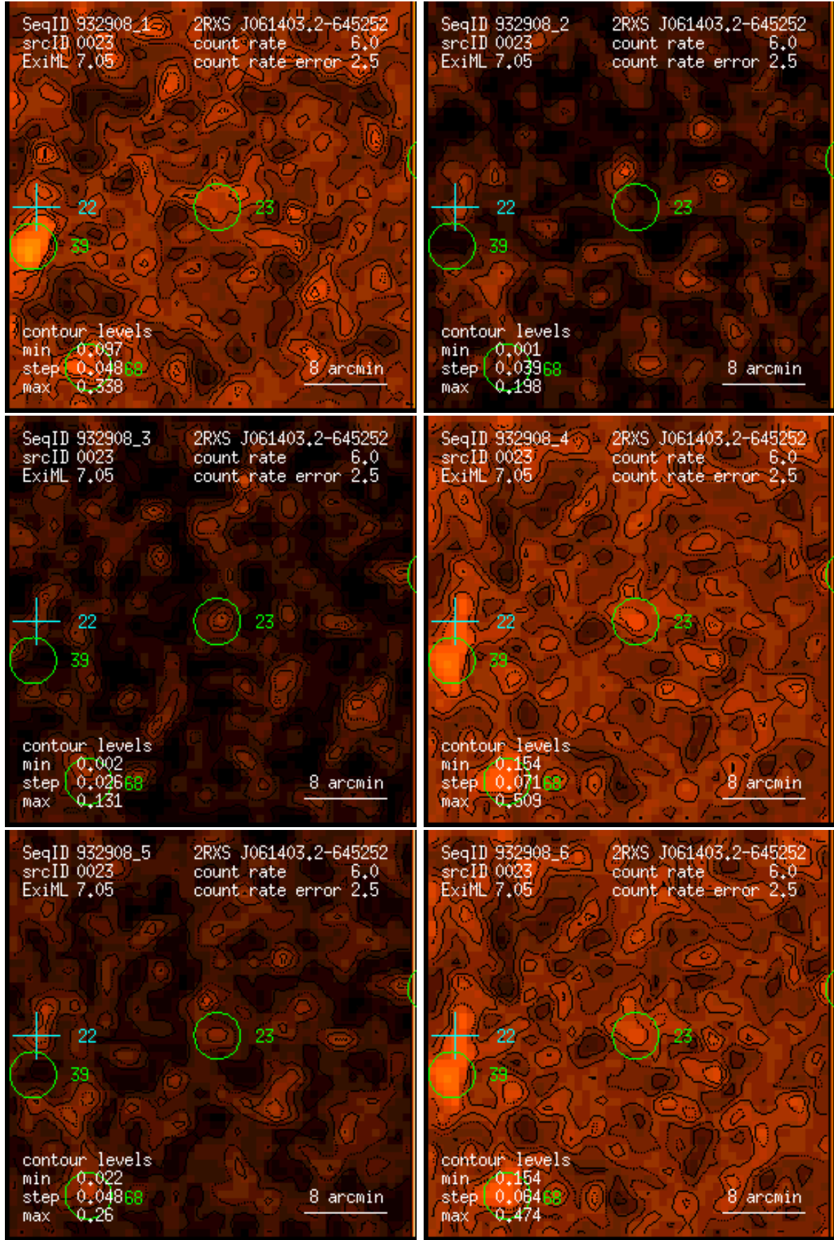
Figure 23: RASS 932908: detection 0023: band rate images, Gaussian filter: (1) PSPC channels 11 – 41, (2) 52 – 90, (3) 91 – 201, (4) 11 – 235, (5) 52 – 201, (6) 11 – 201. Broad band rates in counts/ks. Band rate contour levels in counts/ks/arcmin 2 .
