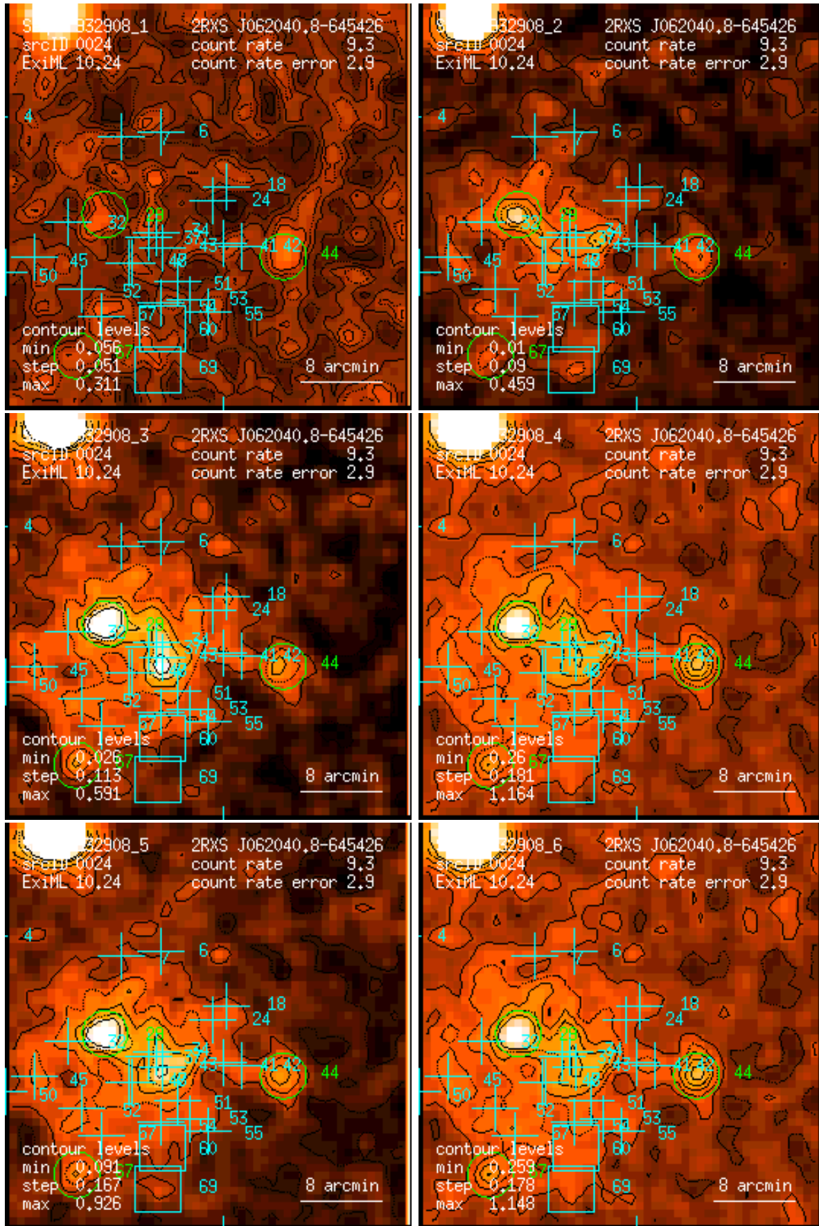
Figure 24: RASS 932908: detection 0024: band rate images, Gaussian filter: (1) PSPC channels 11 – 41, (2) 52 – 90, (3) 91 – 201, (4) 11 – 235, (5) 52 – 201, (6) 11 – 201. Broad band rates in counts/ks. Band rate contour levels in counts/ks/arcmin 2 .
