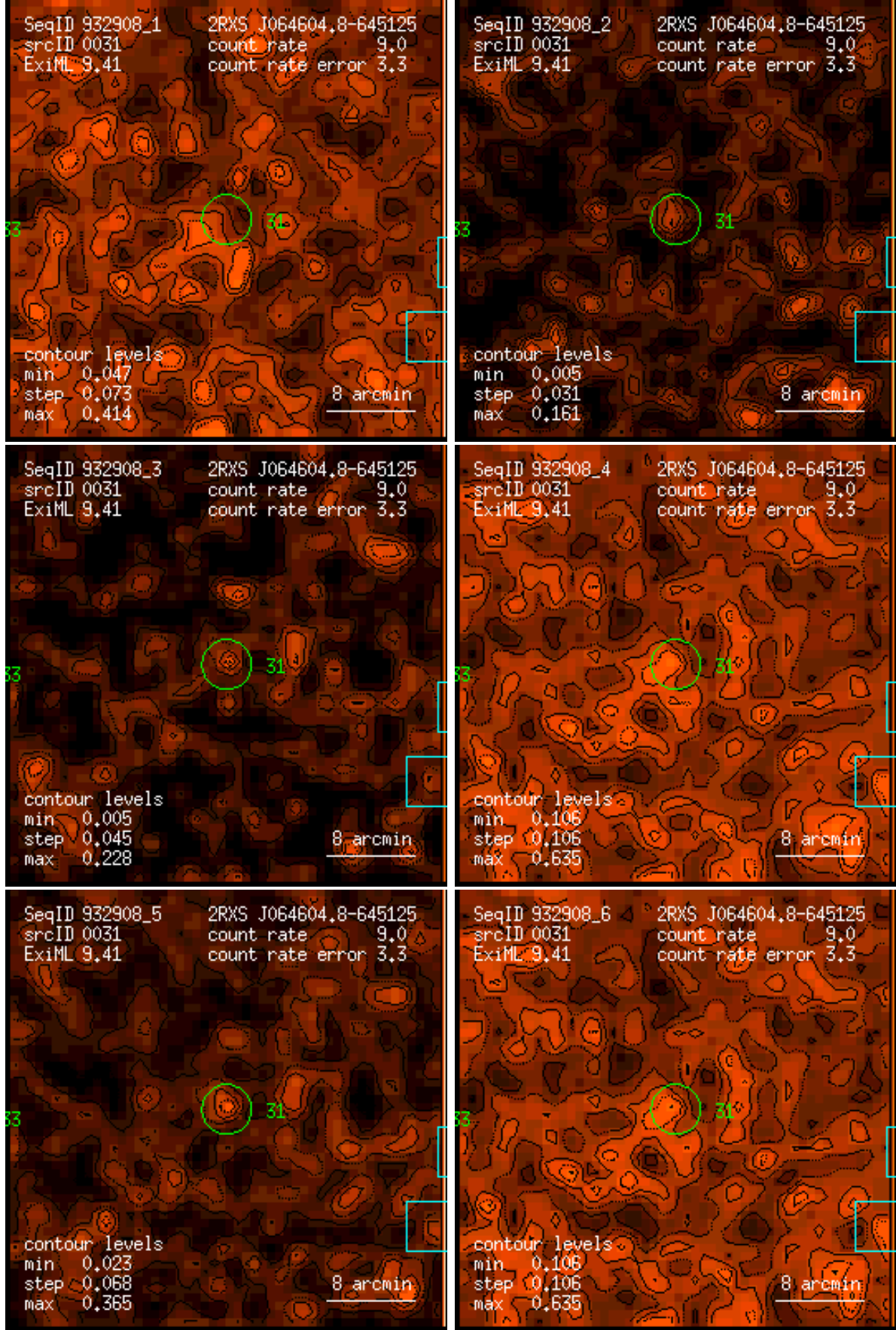
Figure 31: RASS 932908: detection 0031: band rate images, Gaussian filter: (1) PSPC channels 11 – 41, (2) 52 – 90, (3) 91 – 201, (4) 11 – 235, (5) 52 – 201, (6) 11 – 201. Broad band rates in counts/ks. Band rate contour levels in counts/ks/arcmin 2 .
