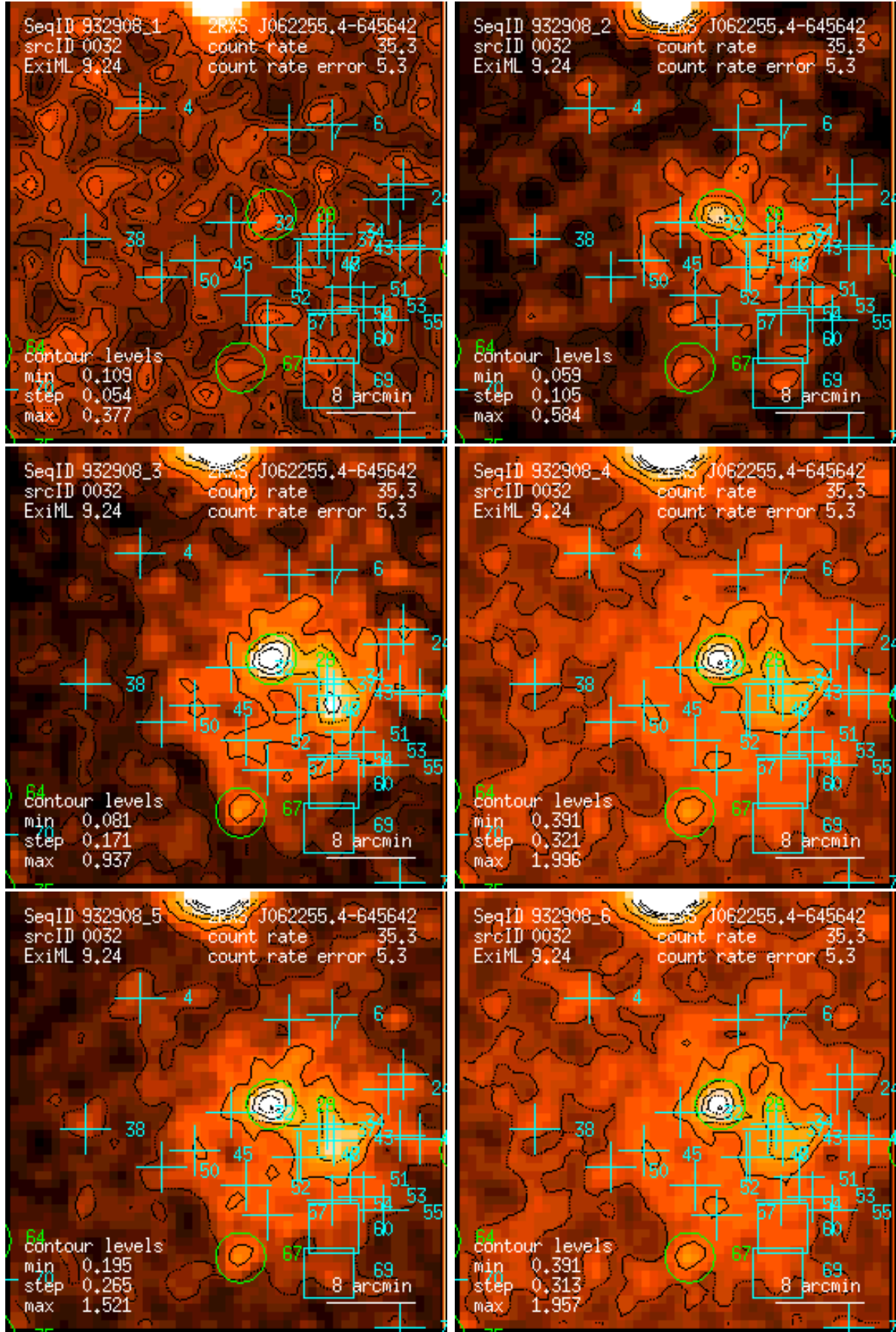
Figure 32: RASS 932908: detection 0032: band rate images, Gaussian filter: (1) PSPC channels 11 – 41, (2) 52 – 90, (3) 91 – 201, (4) 11 – 235, (5) 52 – 201, (6) 11 – 201. Broad band rates in counts/ks. Band rate contour levels in counts/ks/arcmin 2 .
