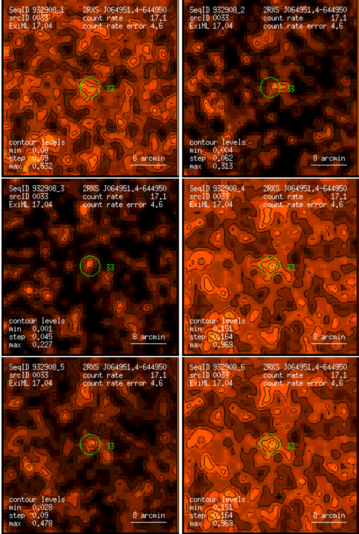
Figure 33: RASS 932908: detection 0033: band rate images, Gaussian filter: (1) PSPC channels 11 – 41, (2) 52 – 90, (3) 91 – 201, (4) 11 – 235, (5) 52 – 201, (6) 11 – 201. Broad band rates in counts/ks. Band rate contour levels in counts/ks/arcmin 2 .
