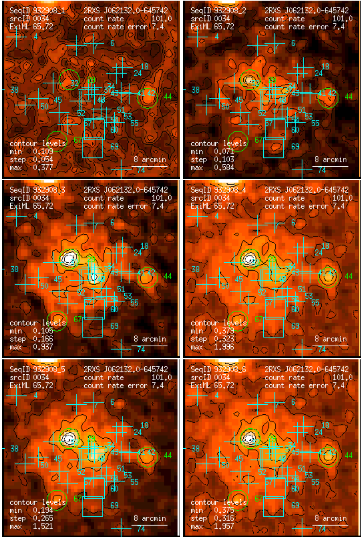
Figure 34: RASS 932908: detection 0034: band rate images, Gaussian filter: (1) PSPC channels 11 – 41, (2) 52 – 90, (3) 91 – 201, (4) 11 – 235, (5) 52 – 201, (6) 11 – 201. Broad band rates in counts/ks. Band rate contour levels in counts/ks/arcmin 2 .
