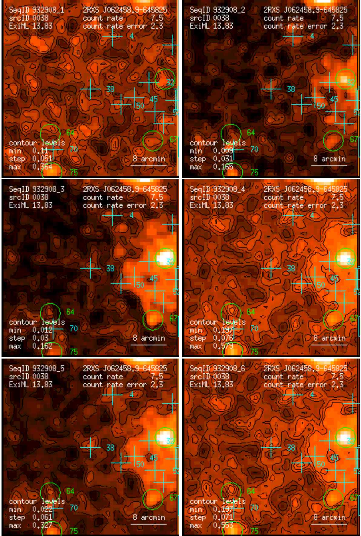
Figure 38: RASS 932908: detection 0038: band rate images, Gaussian filter: (1) PSPC channels 11 – 41, (2) 52 – 90, (3) 91 – 201, (4) 11 – 235, (5) 52 – 201, (6) 11 – 201. Broad band rates in counts/ks. Band rate contour levels in counts/ks/arcmin 2 .
