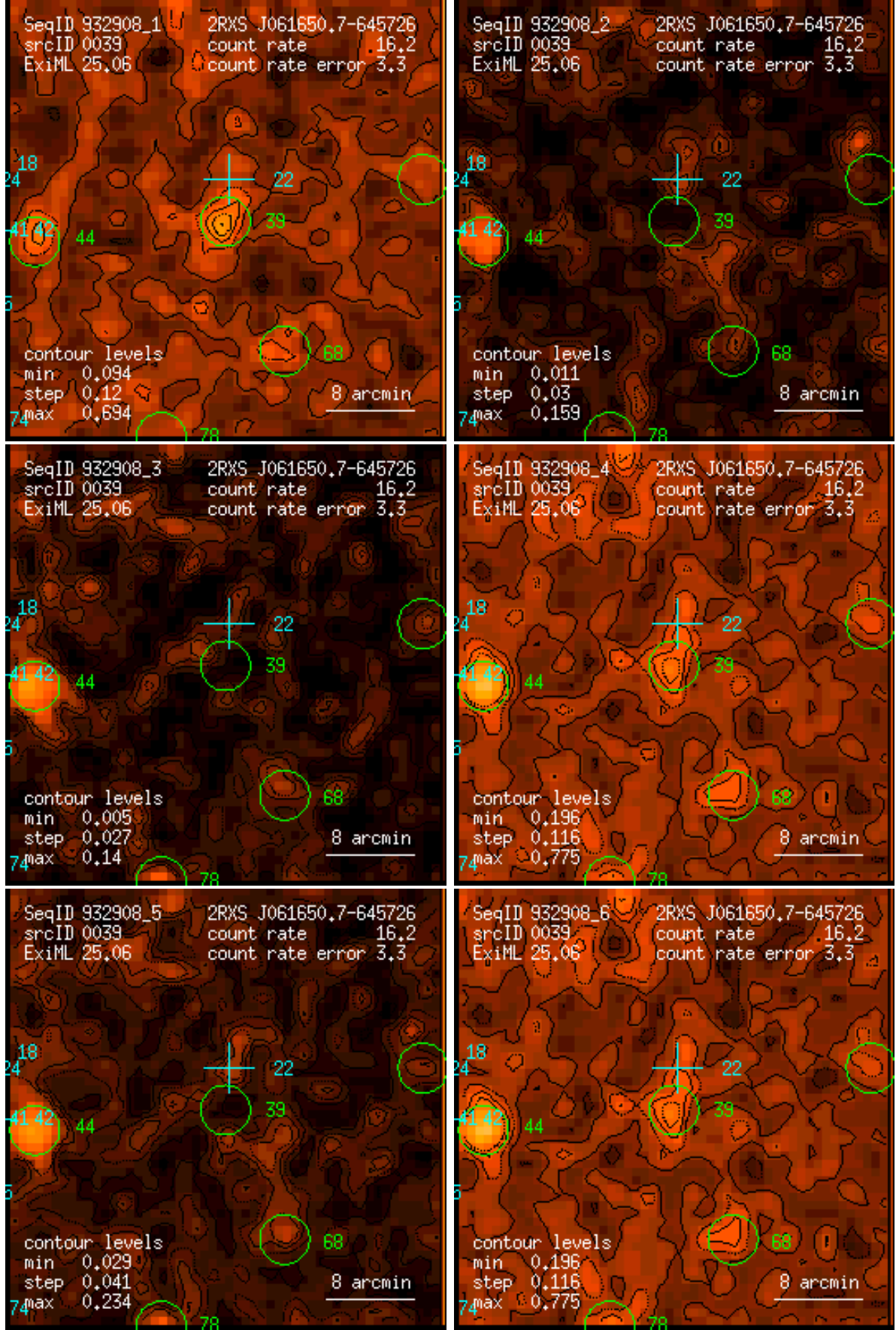
Figure 39: RASS 932908: detection 0039: band rate images, Gaussian filter: (1) PSPC channels 11 – 41, (2) 52 – 90, (3) 91 – 201, (4) 11 – 235, (5) 52 – 201, (6) 11 – 201. Broad band rates in counts/ks. Band rate contour levels in counts/ks/arcmin 2 .
