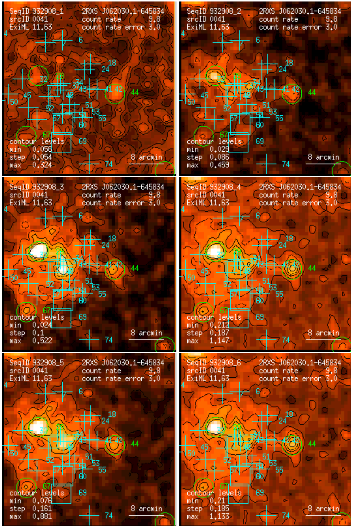
Figure 41: RASS 932908: detection 0041: band rate images, Gaussian filter: (1) PSPC channels 11 – 41, (2) 52 – 90, (3) 91 – 201, (4) 11 – 235, (5) 52 – 201, (6) 11 – 201. Broad band rates in counts/ks. Band rate contour levels in counts/ks/arcmin 2 .
