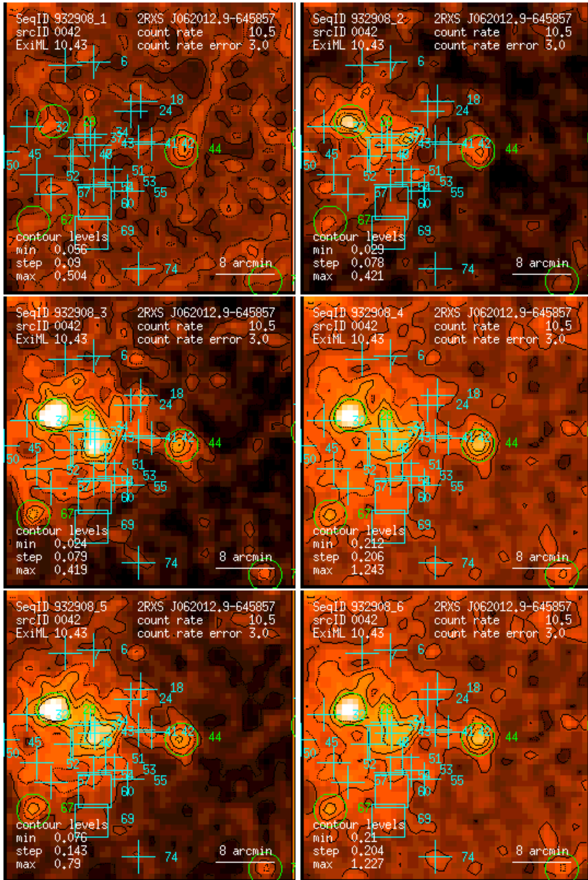
Figure 42: RASS 932908: detection 0042: band rate images, Gaussian filter: (1) PSPC channels 11 – 41, (2) 52 – 90, (3) 91 – 201, (4) 11 – 235, (5) 52 – 201, (6) 11 – 201. Broad band rates in counts/ks. Band rate contour levels in counts/ks/arcmin 2 .
