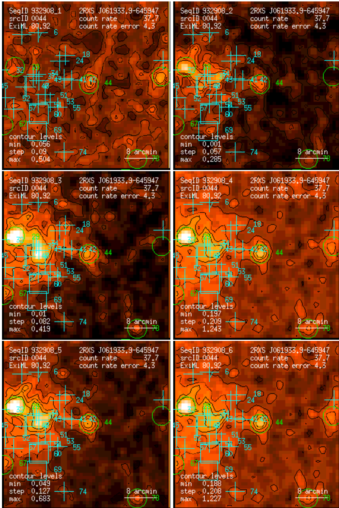
Figure 44: RASS 932908: detection 0044: band rate images, Gaussian filter: (1) PSPC channels 11 – 41, (2) 52 – 90, (3) 91 – 201, (4) 11 – 235, (5) 52 – 201, (6) 11 – 201. Broad band rates in counts/ks. Band rate contour levels in counts/ks/arcmin 2 .
