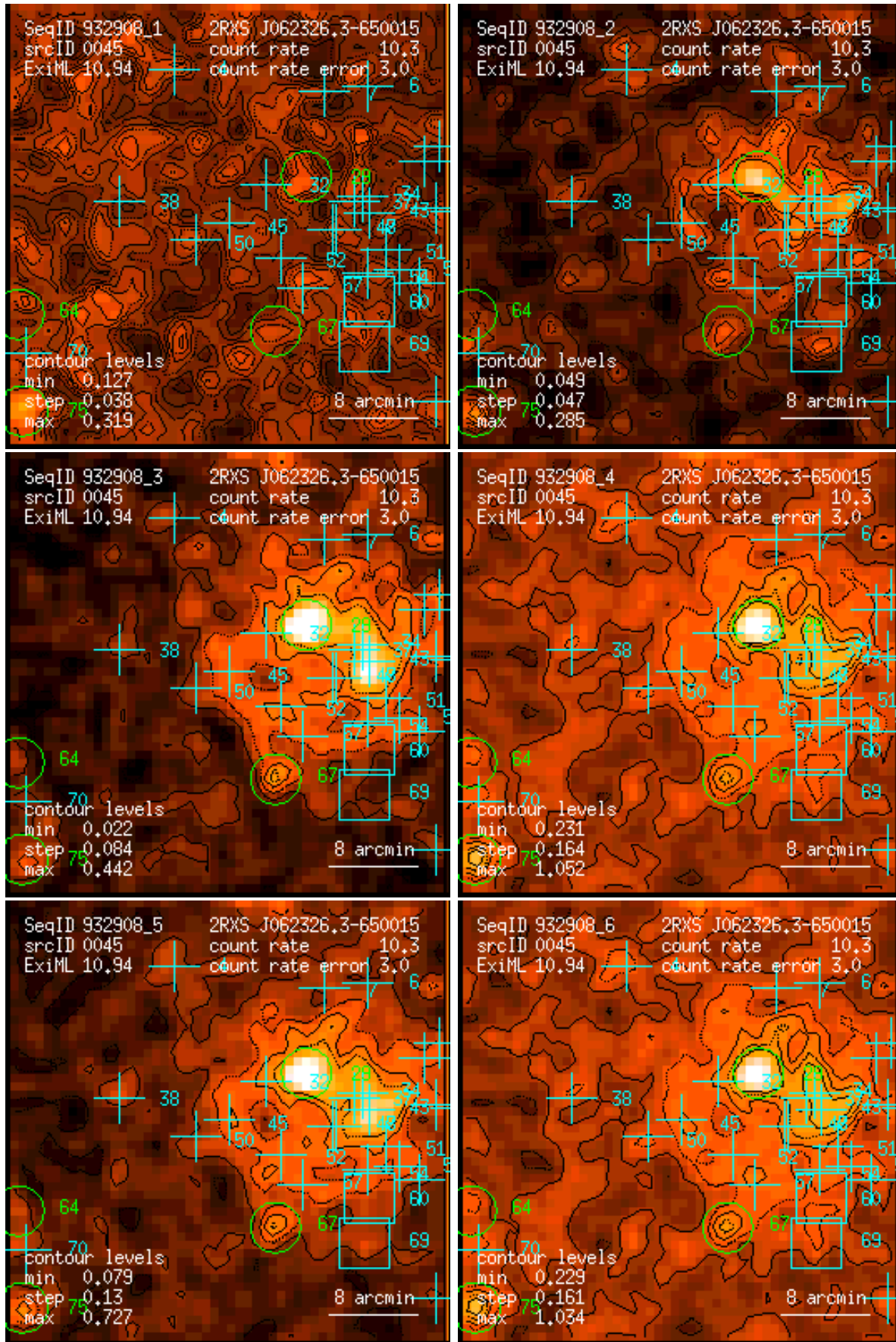
Figure 45: RASS 932908: detection 0045: band rate images, Gaussian filter: (1) PSPC channels 11 – 41, (2) 52 – 90, (3) 91 – 201, (4) 11 – 235, (5) 52 – 201, (6) 11 – 201. Broad band rates in counts/ks. Band rate contour levels in counts/ks/arcmin 2 .
