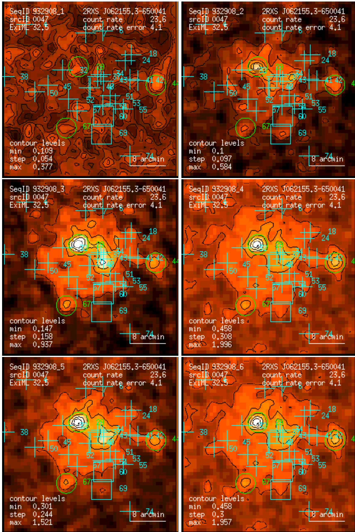
Figure 47: RASS 932908: detection 0047: band rate images, Gaussian filter: (1) PSPC channels 11 – 41, (2) 52 – 90, (3) 91 – 201, (4) 11 – 235, (5) 52 – 201, (6) 11 – 201. Broad band rates in counts/ks. Band rate contour levels in counts/ks/arcmin 2 .
