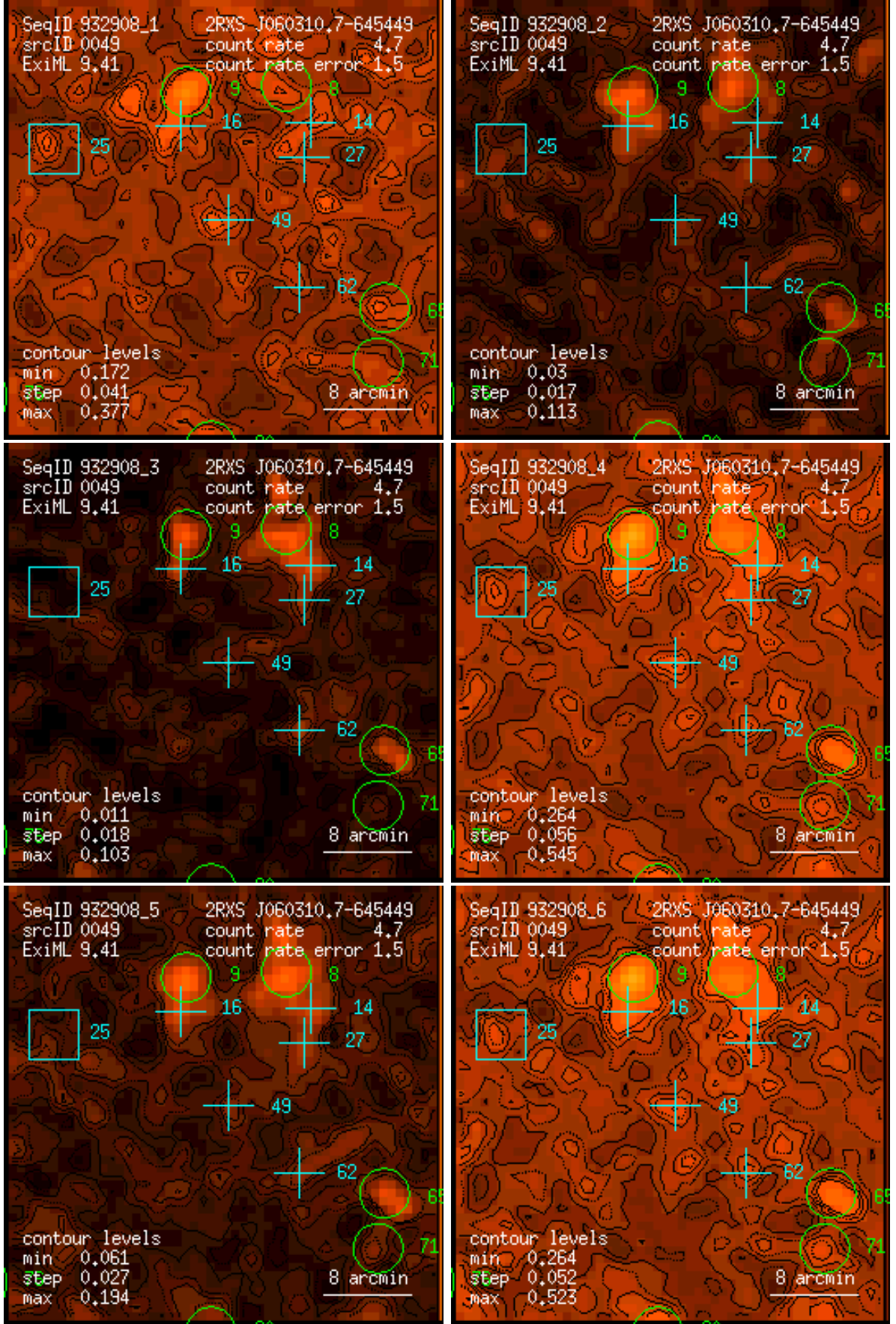
Figure 49: RASS 932908: detection 0049: band rate images, Gaussian filter: (1) PSPC channels 11 – 41, (2) 52 – 90, (3) 91 – 201, (4) 11 – 235, (5) 52 – 201, (6) 11 – 201. Broad band rates in counts/ks. Band rate contour levels in counts/ks/arcmin 2 .
