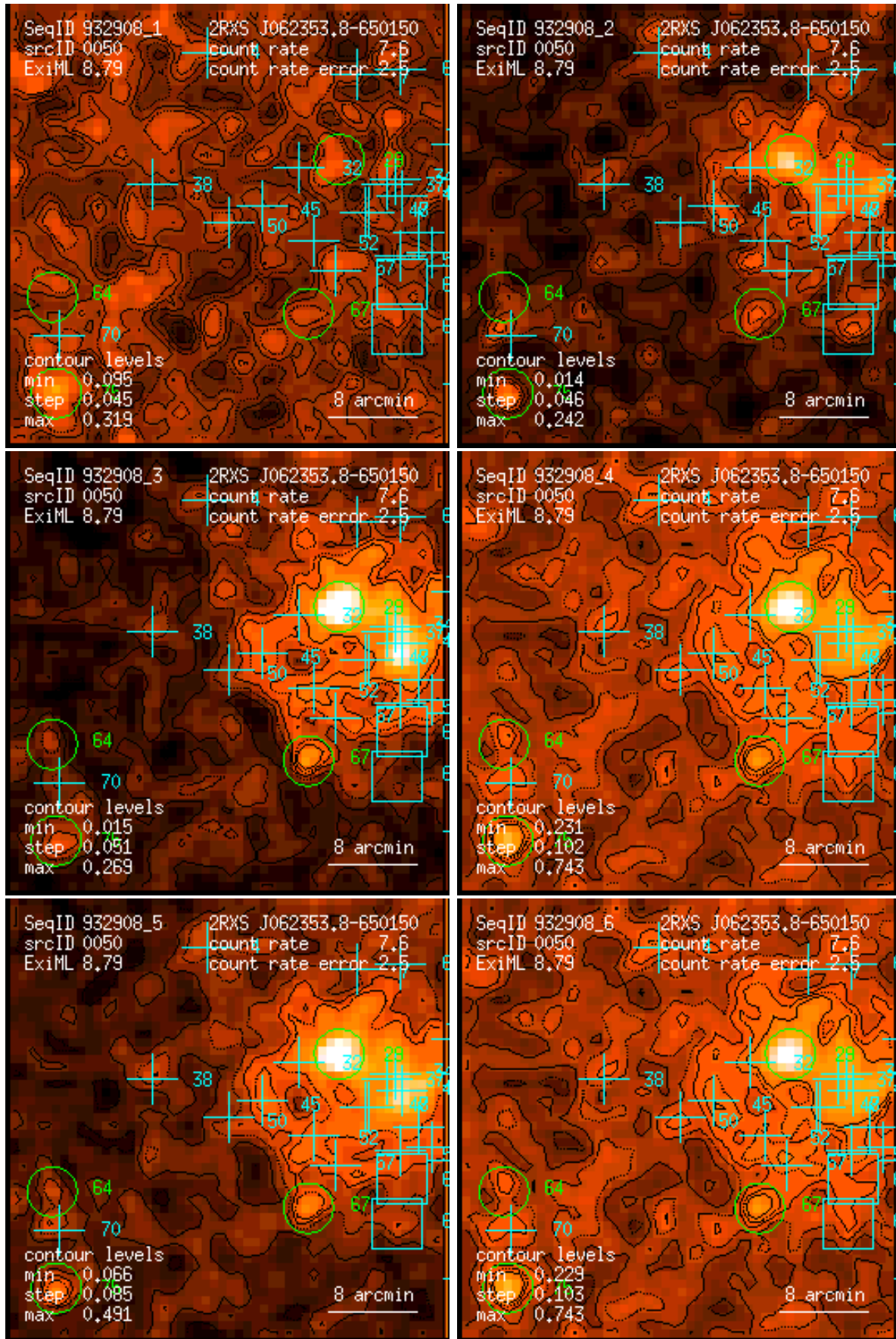
Figure 50: RASS 932908: detection 0050: band rate images, Gaussian filter: (1) PSPC channels 11 – 41, (2) 52 – 90, (3) 91 – 201, (4) 11 – 235, (5) 52 – 201, (6) 11 – 201. Broad band rates in counts/ks. Band rate contour levels in counts/ks/arcmin 2 .
