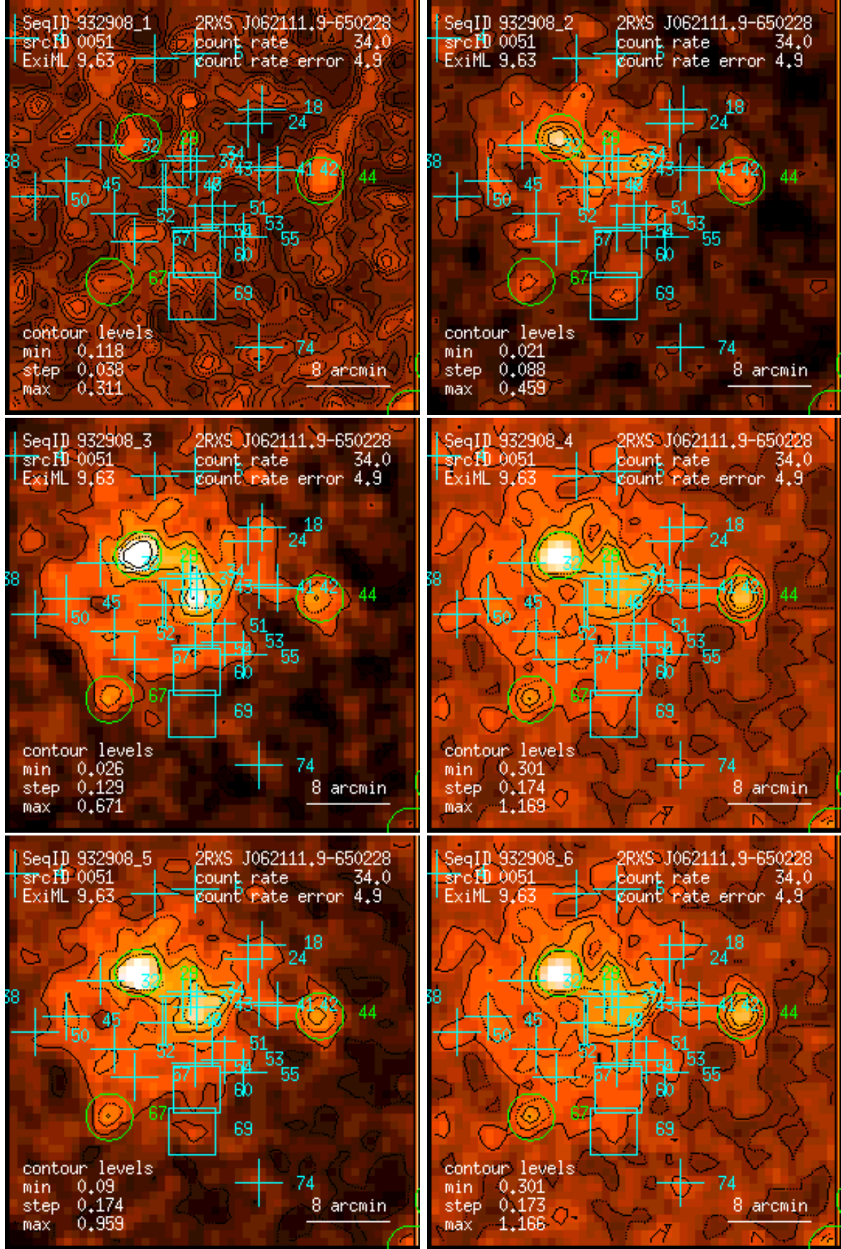
Figure 51: RASS 932908: detection 0051: band rate images, Gaussian filter: (1) PSPC channels 11 – 41, (2) 52 – 90, (3) 91 – 201, (4) 11 – 235, (5) 52 – 201, (6) 11 – 201. Broad band rates in counts/ks. Band rate contour levels in counts/ks/arcmin 2 .
