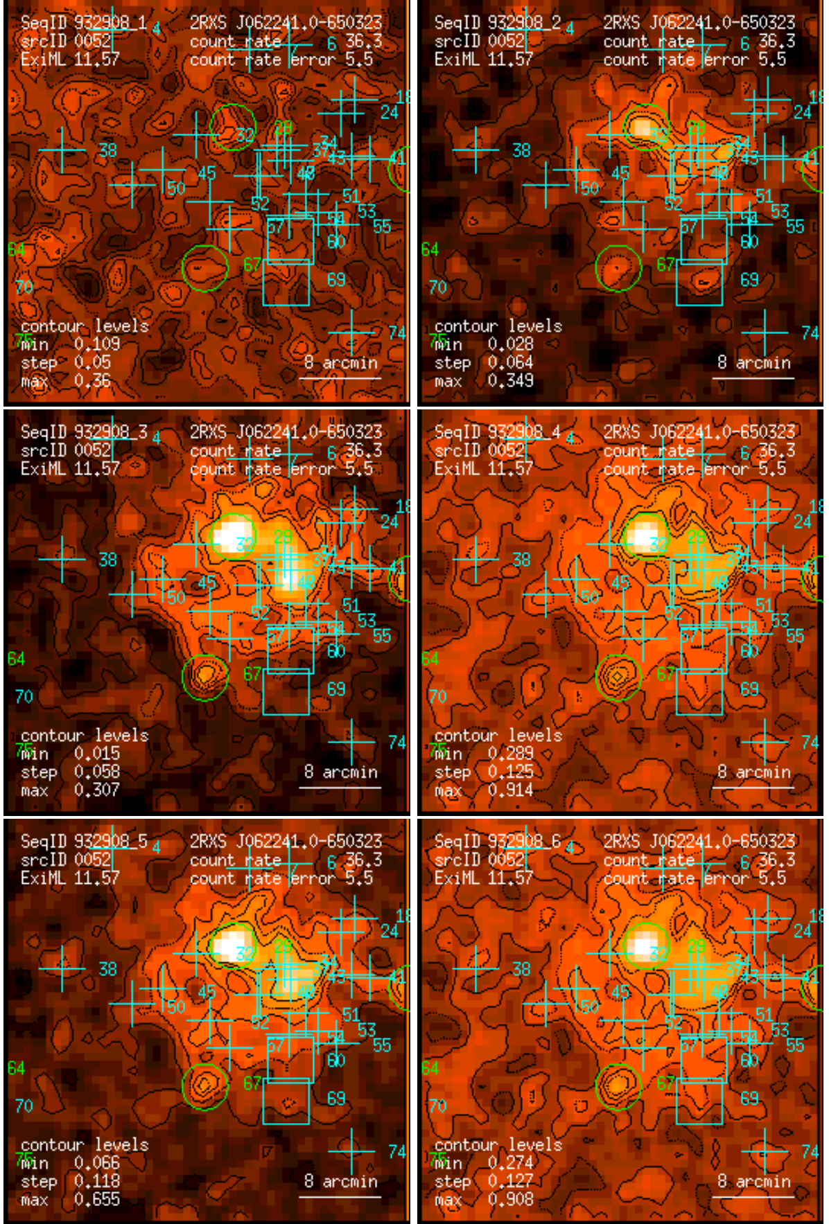
Figure 52: RASS 932908: detection 0052: band rate images, Gaussian filter: (1) PSPC channels 11 – 41, (2) 52 – 90, (3) 91 – 201, (4) 11 – 235, (5) 52 – 201, (6) 11 – 201. Broad band rates in counts/ks. Band rate contour levels in counts/ks/arcmin 2 .
