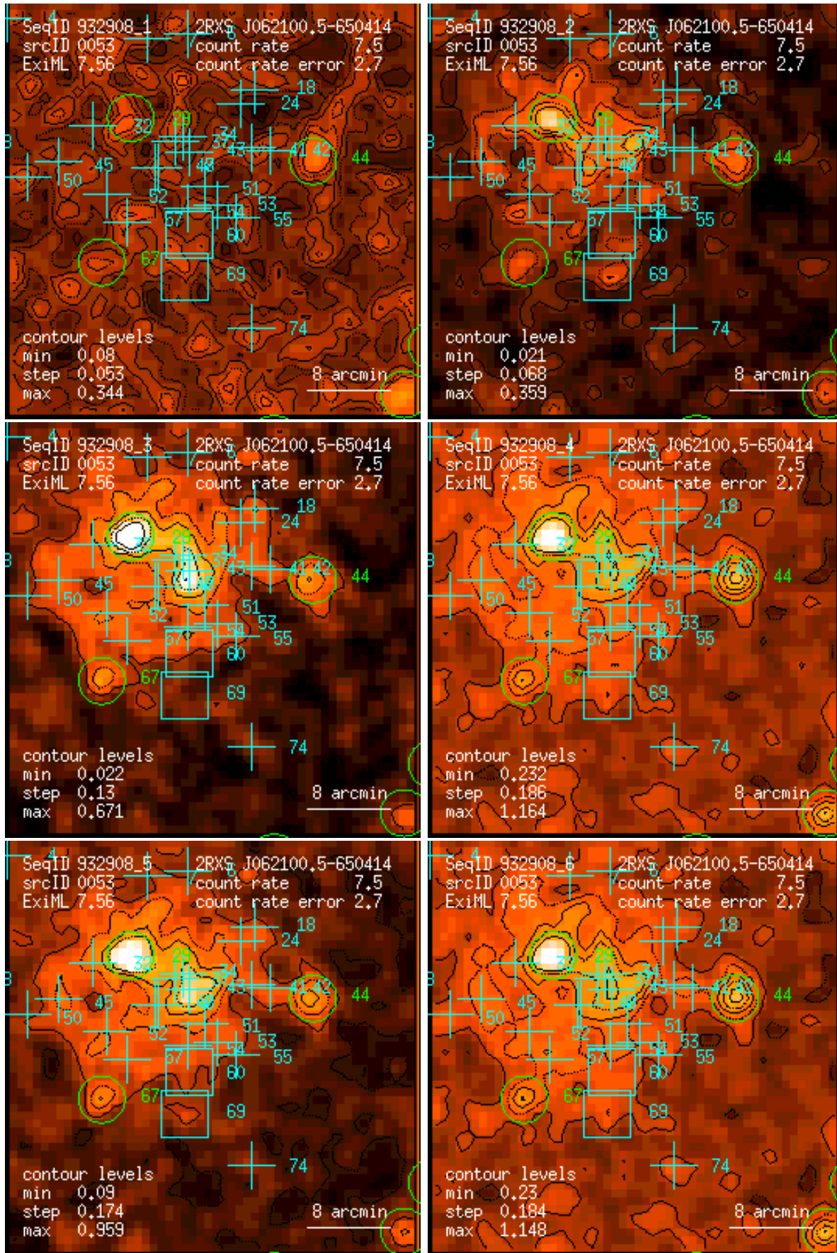
Figure 53: RASS 932908: detection 0053: band rate images, Gaussian filter: (1) PSPC channels 11 – 41, (2) 52 – 90, (3) 91 – 201, (4) 11 – 235, (5) 52 – 201, (6) 11 – 201. Broad band rates in counts/ks. Band rate contour levels in counts/ks/arcmin 2 .
