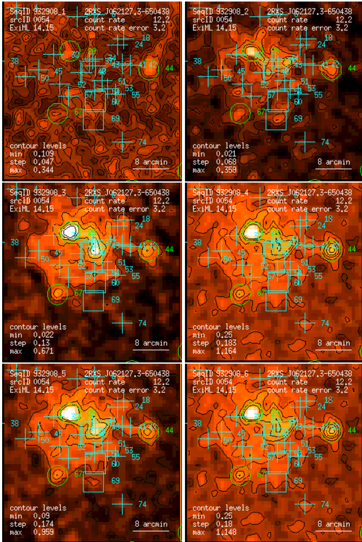
Figure 54: RASS 932908: detection 0054: band rate images, Gaussian filter: (1) PSPC channels 11 – 41, (2) 52 – 90, (3) 91 – 201, (4) 11 – 235, (5) 52 – 201, (6) 11 – 201. Broad band rates in counts/ks. Band rate contour levels in counts/ks/arcmin 2 .
