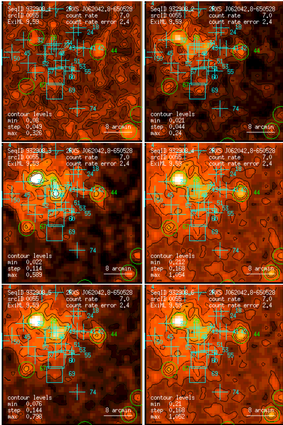
Figure 55: RASS 932908: detection 0055: band rate images, Gaussian filter: (1) PSPC channels 11 – 41, (2) 52 – 90, (3) 91 – 201, (4) 11 – 235, (5) 52 – 201, (6) 11 – 201. Broad band rates in counts/ks. Band rate contour levels in counts/ks/arcmin 2 .
