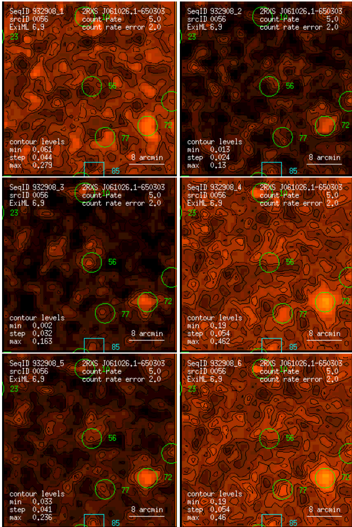
Figure 56: RASS 932908: detection 0056: band rate images, Gaussian filter: (1) PSPC channels 11 – 41, (2) 52 – 90, (3) 91 – 201, (4) 11 – 235, (5) 52 – 201, (6) 11 – 201. Broad band rates in counts/ks. Band rate contour levels in counts/ks/arcmin 2 .
