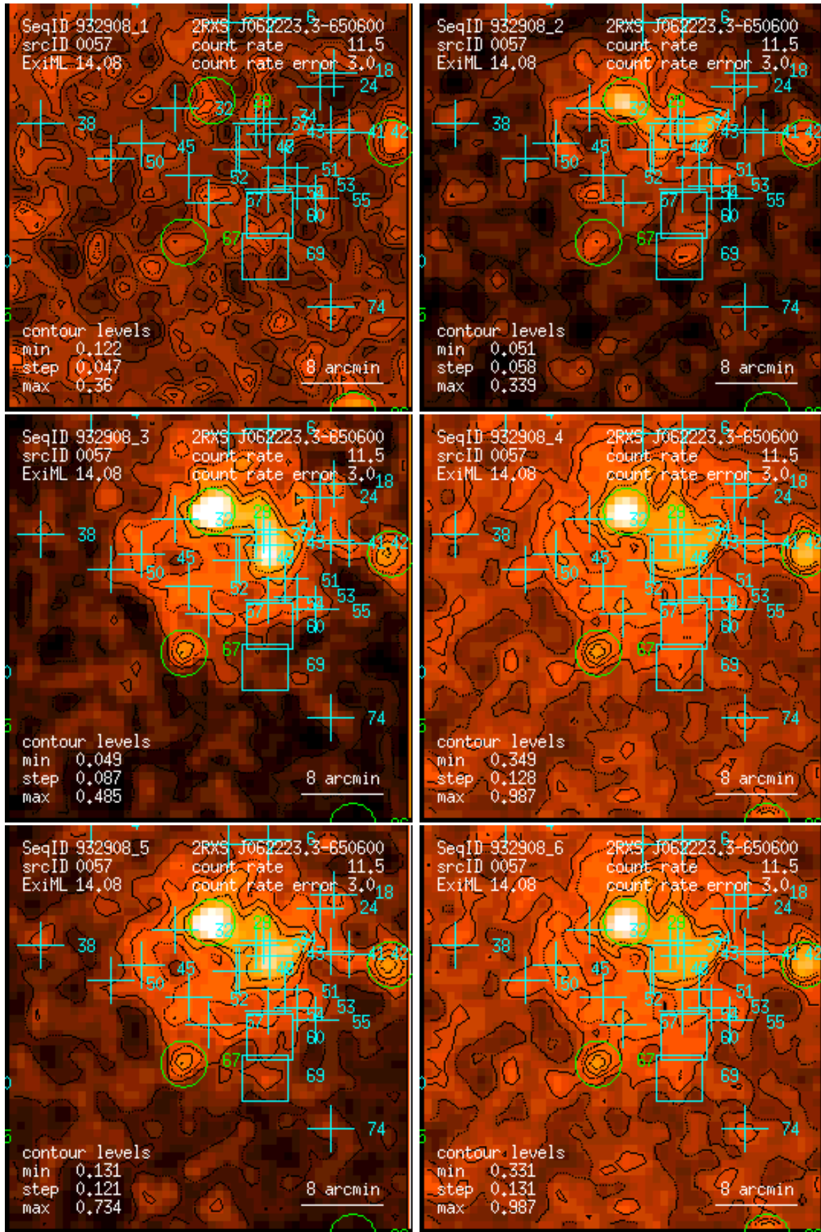
Figure 57: RASS 932908: detection 0057: band rate images, Gaussian filter: (1) PSPC channels 11 – 41, (2) 52 – 90, (3) 91 – 201, (4) 11 – 235, (5) 52 – 201, (6) 11 – 201. Broad band rates in counts/ks. Band rate contour levels in counts/ks/arcmin 2 .
