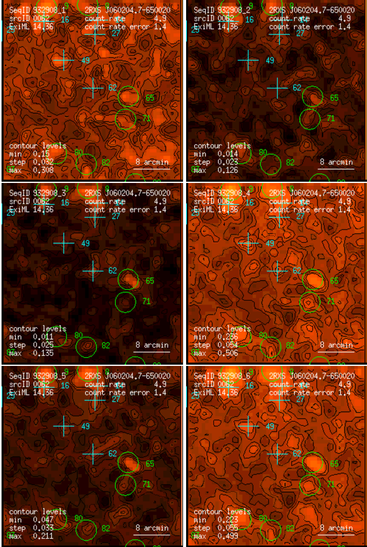
Figure 62: RASS 932908: detection 0062: band rate images, Gaussian filter: (1) PSPC channels 11 – 41, (2) 52 – 90, (3) 91 – 201, (4) 11 – 235, (5) 52 – 201, (6) 11 – 201. Broad band rates in counts/ks. Band rate contour levels in counts/ks/arcmin 2 .
