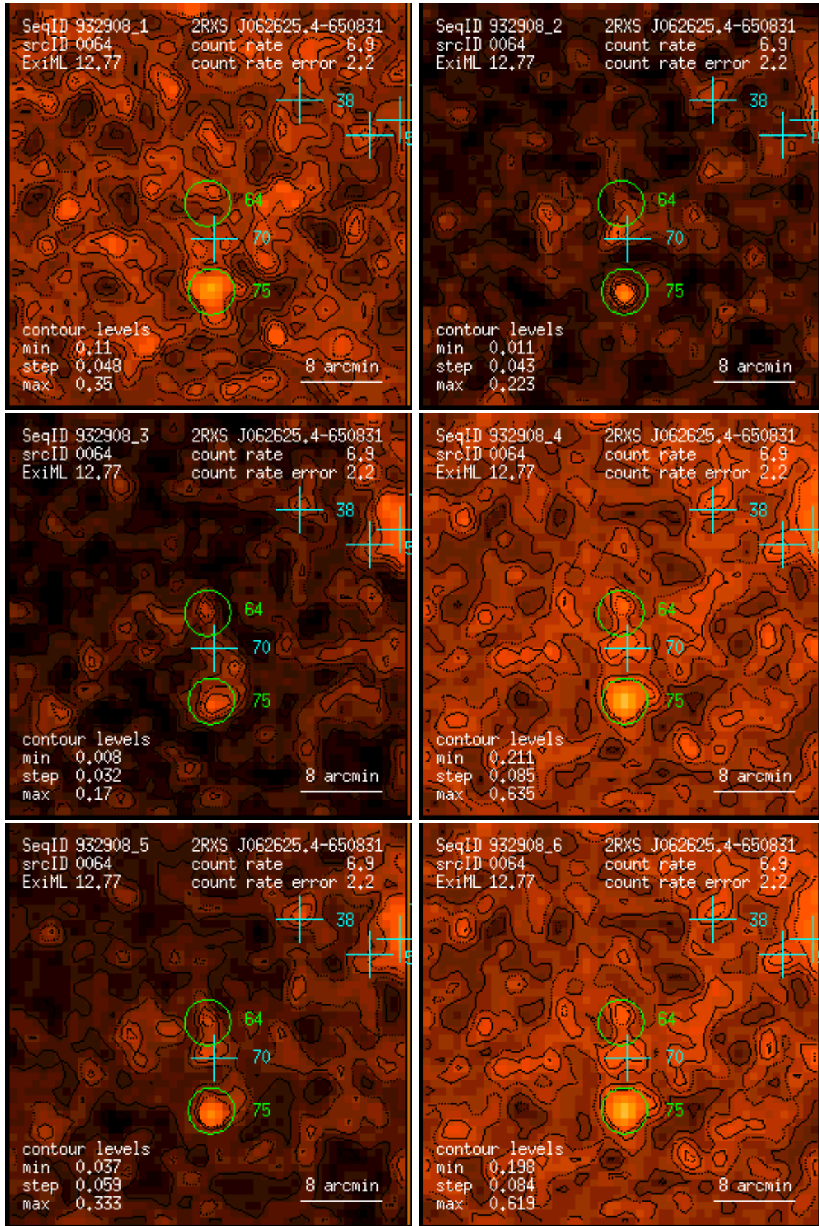
Figure 64: RASS 932908: detection 0064: band rate images, Gaussian filter: (1) PSPC channels 11 – 41, (2) 52 – 90, (3) 91 – 201, (4) 11 – 235, (5) 52 – 201, (6) 11 – 201. Broad band rates in counts/ks. Band rate contour levels in counts/ks/arcmin 2 .
