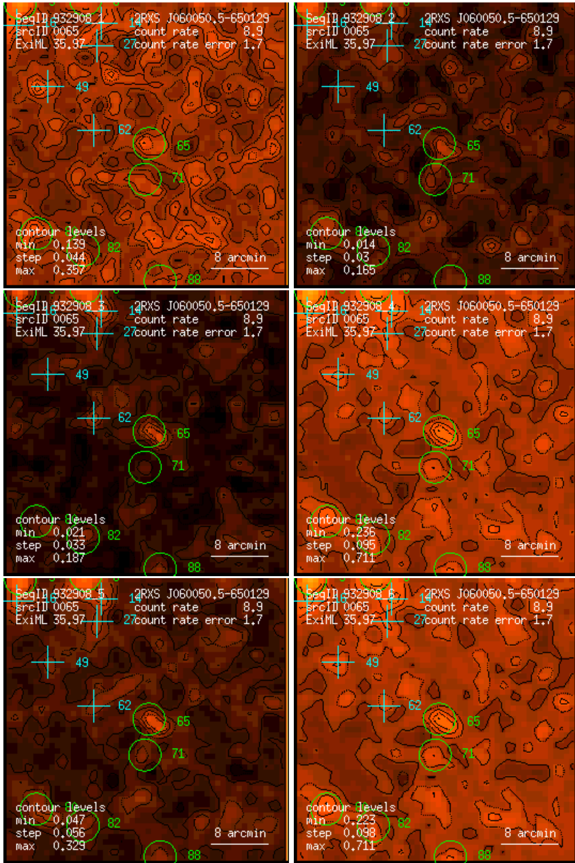
Figure 65: RASS 932908: detection 0065: band rate images, Gaussian filter: (1) PSPC channels 11 – 41, (2) 52 – 90, (3) 91 – 201, (4) 11 – 235, (5) 52 – 201, (6) 11 – 201. Broad band rates in counts/ks. Band rate contour levels in counts/ks/arcmin 2 .
