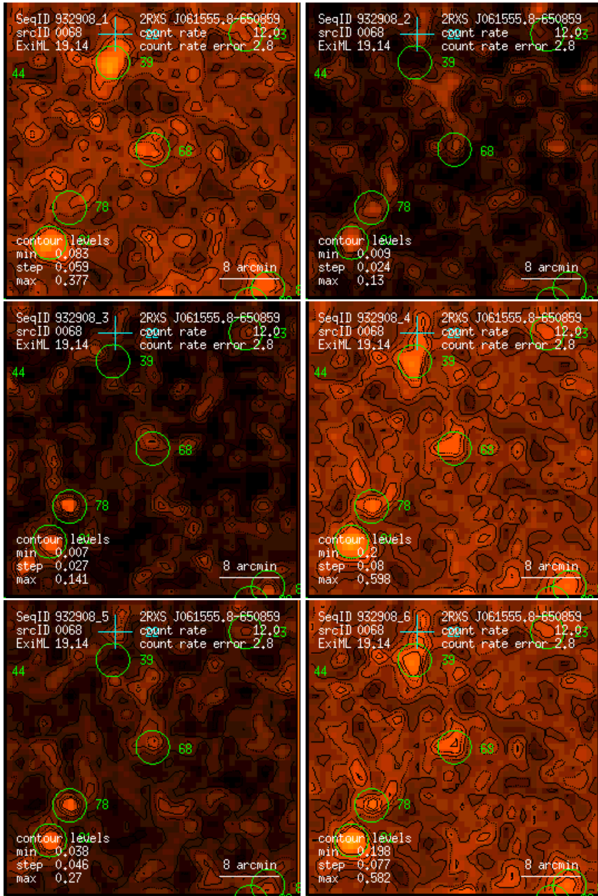
Figure 68: RASS 932908: detection 0068: band rate images, Gaussian filter: (1) PSPC channels 11 – 41, (2) 52 – 90, (3) 91 – 201, (4) 11 – 235, (5) 52 – 201, (6) 11 – 201. Broad band rates in counts/ks. Band rate contour levels in counts/ks/arcmin 2 .
