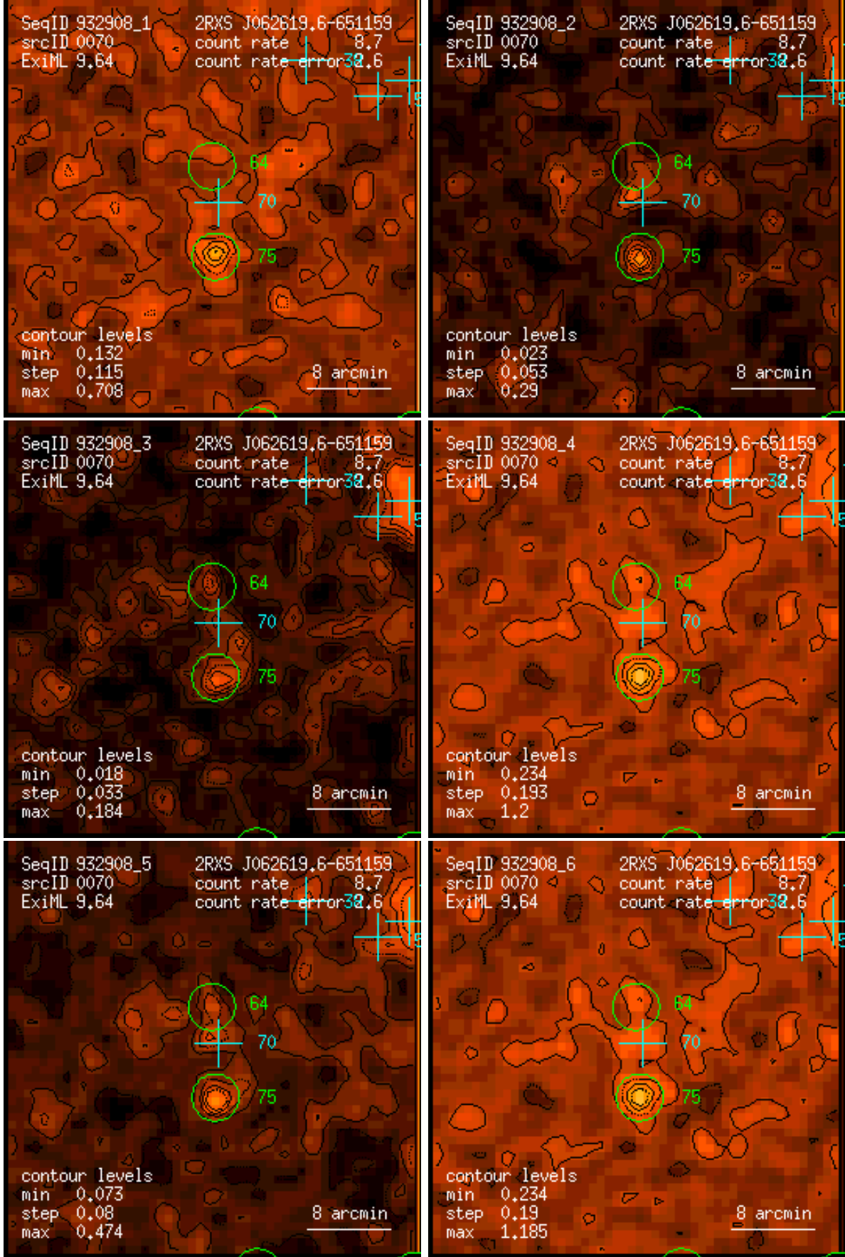
Figure 70: RASS 932908: detection 0070: band rate images, Gaussian filter: (1) PSPC channels 11 – 41, (2) 52 – 90, (3) 91 – 201, (4) 11 – 235, (5) 52 – 201, (6) 11 – 201. Broad band rates in counts/ks. Band rate contour levels in counts/ks/arcmin 2 .
