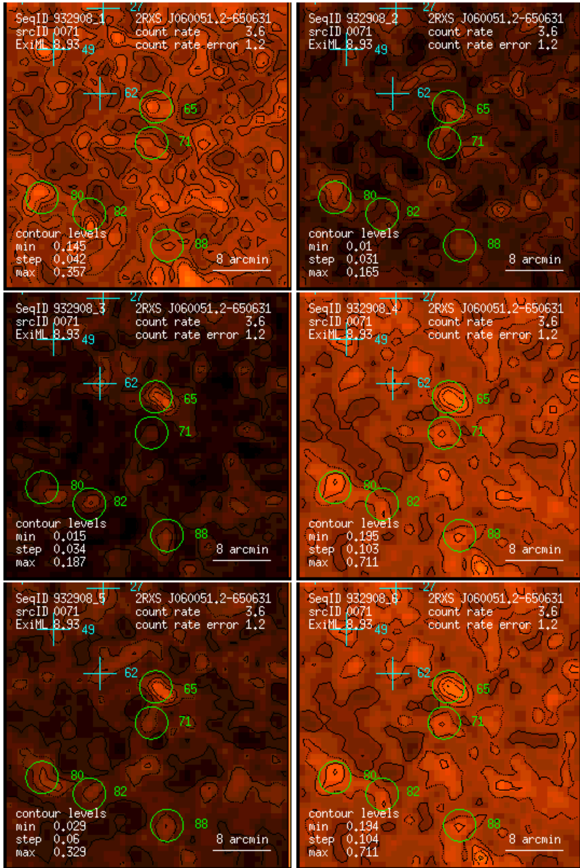
Figure 71: RASS 932908: detection 0071: band rate images, Gaussian filter: (1) PSPC channels 11 – 41, (2) 52 – 90, (3) 91 – 201, (4) 11 – 235, (5) 52 – 201, (6) 11 – 201. Broad band rates in counts/ks. Band rate contour levels in counts/ks/arcmin 2 .
