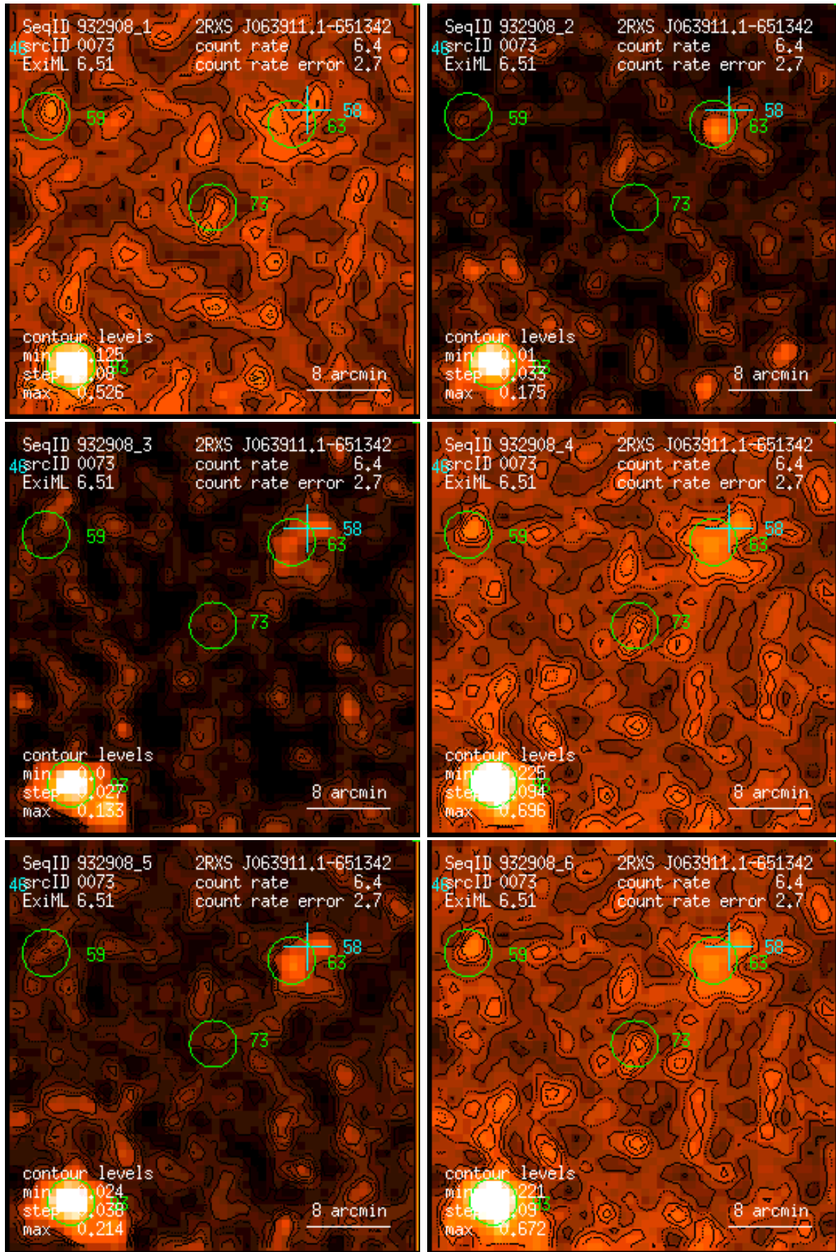
Figure 73: RASS 932908: detection 0073: band rate images, Gaussian filter: (1) PSPC channels 11 – 41, (2) 52 – 90, (3) 91 – 201, (4) 11 – 235, (5) 52 – 201, (6) 11 – 201. Broad band rates in counts/ks. Band rate contour levels in counts/ks/arcmin 2 .
