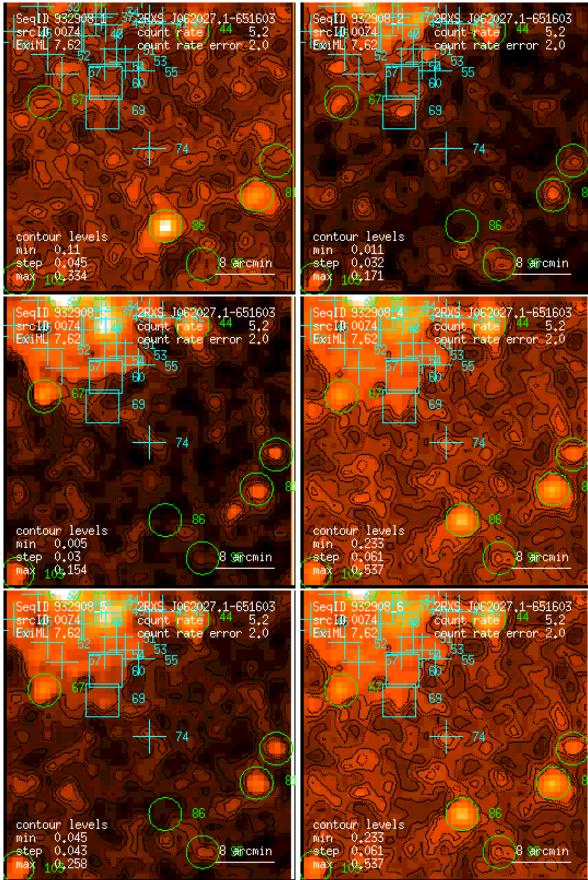
Figure 74: RASS 932908: detection 0074: band rate images, Gaussian filter: (1) PSPC channels 11 – 41, (2) 52 – 90, (3) 91 – 201, (4) 11 – 235, (5) 52 – 201, (6) 11 – 201. Broad band rates in counts/ks. Band rate contour levels in counts/ks/arcmin 2 .
