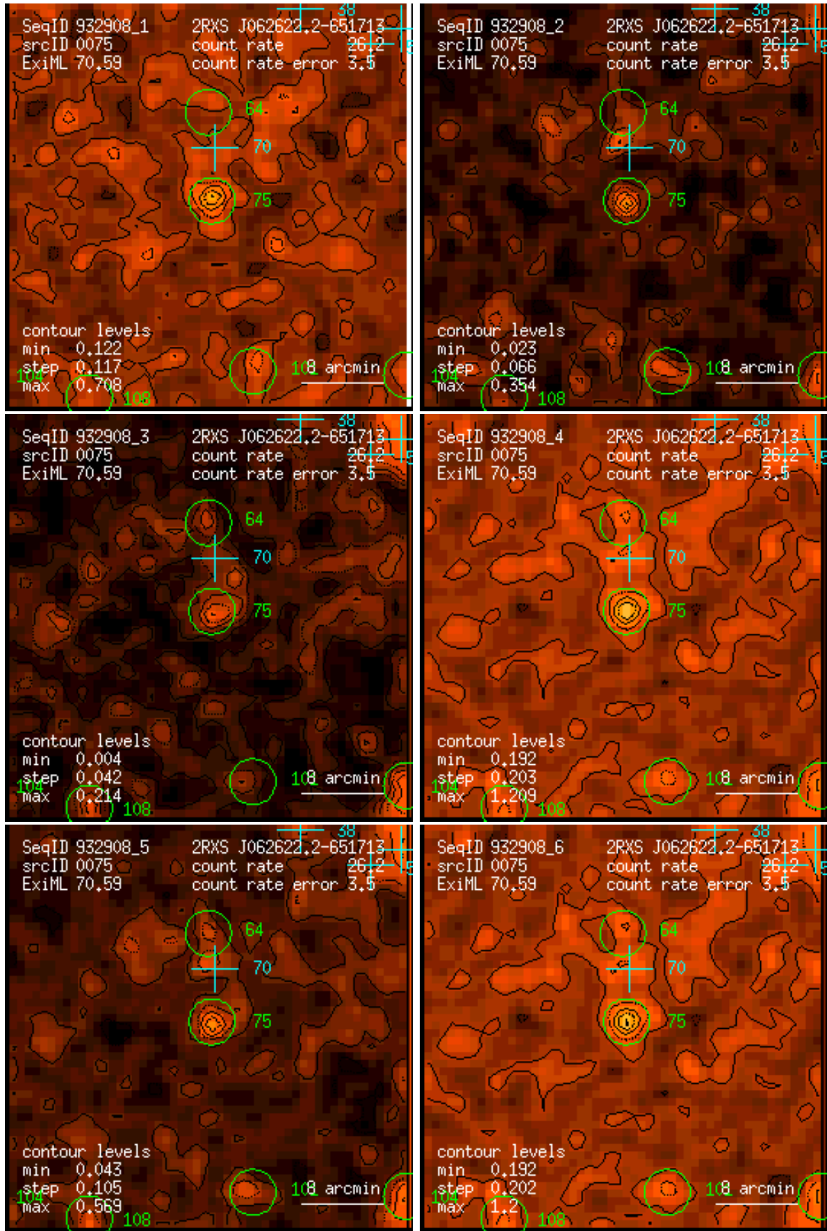
Figure 75: RASS 932908: detection 0075: band rate images, Gaussian filter: (1) PSPC channels 11 – 41, (2) 52 – 90, (3) 91 – 201, (4) 11 – 235, (5) 52 – 201, (6) 11 – 201. Broad band rates in counts/ks. Band rate contour levels in counts/ks/arcmin 2 .
