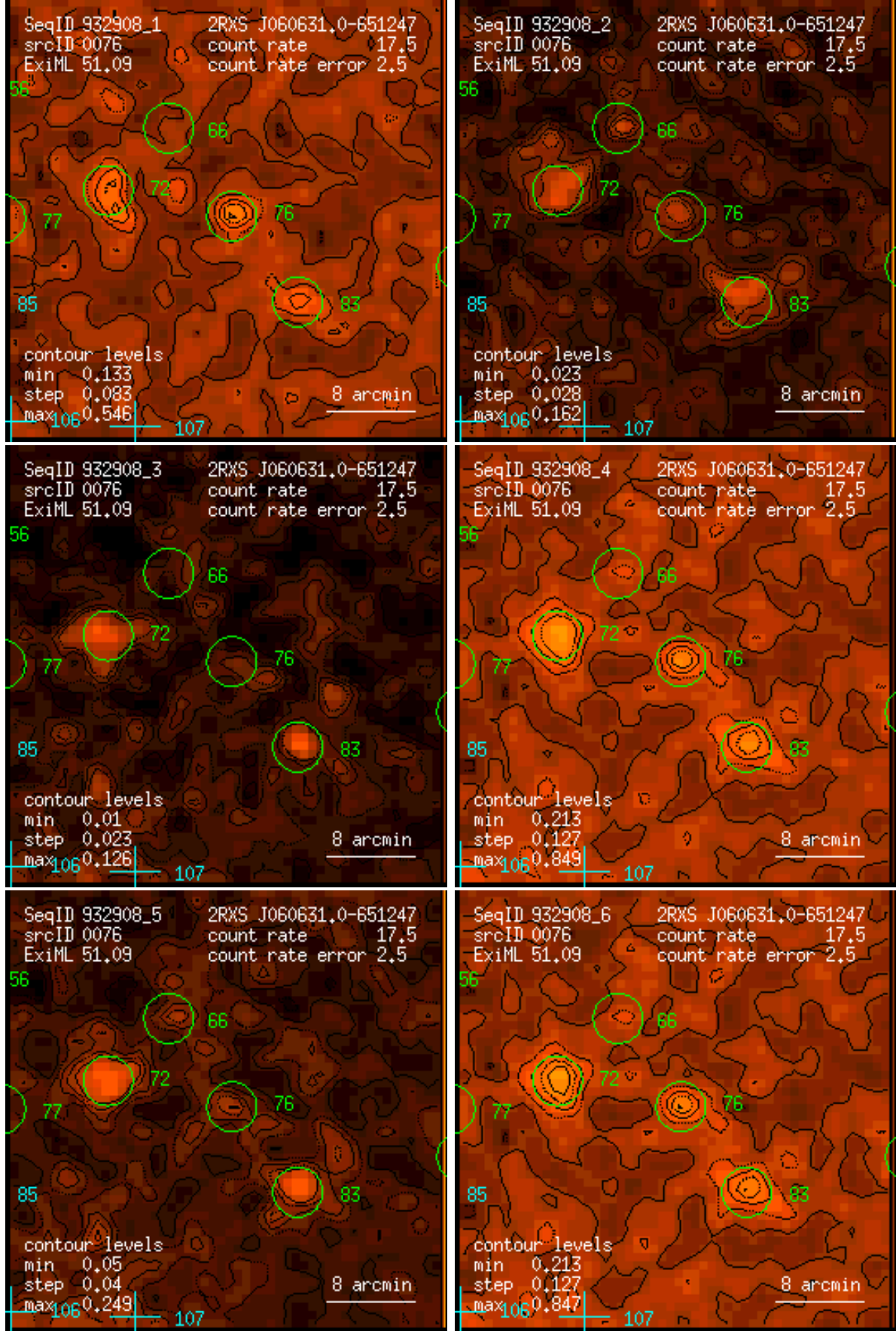
Figure 76: RASS 932908: detection 0076: band rate images, Gaussian filter: (1) PSPC channels 11 – 41, (2) 52 – 90, (3) 91 – 201, (4) 11 – 235, (5) 52 – 201, (6) 11 – 201. Broad band rates in counts/ks. Band rate contour levels in counts/ks/arcmin 2 .
