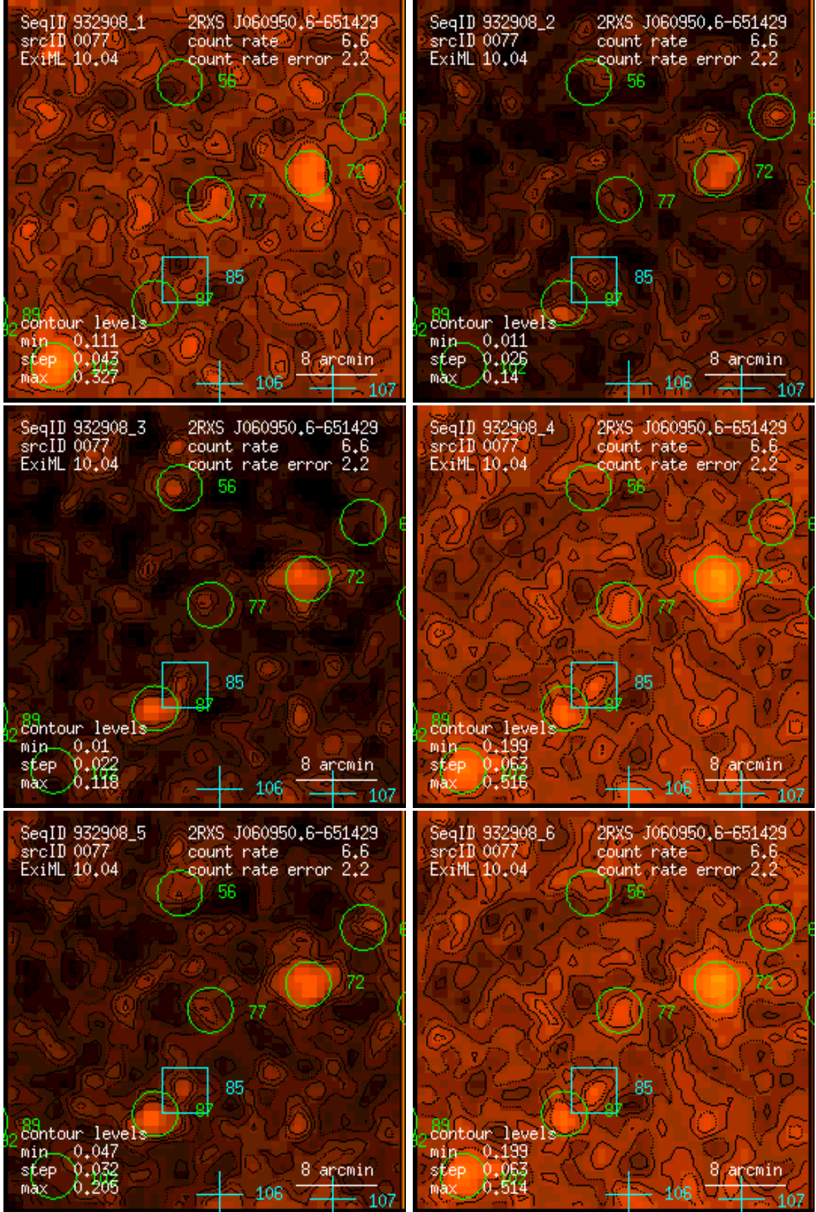
Figure 77: RASS 932908: detection 0077: band rate images, Gaussian filter: (1) PSPC channels 11 – 41, (2) 52 – 90, (3) 91 – 201, (4) 11 – 235, (5) 52 – 201, (6) 11 – 201. Broad band rates in counts/ks. Band rate contour levels in counts/ks/arcmin 2 .
