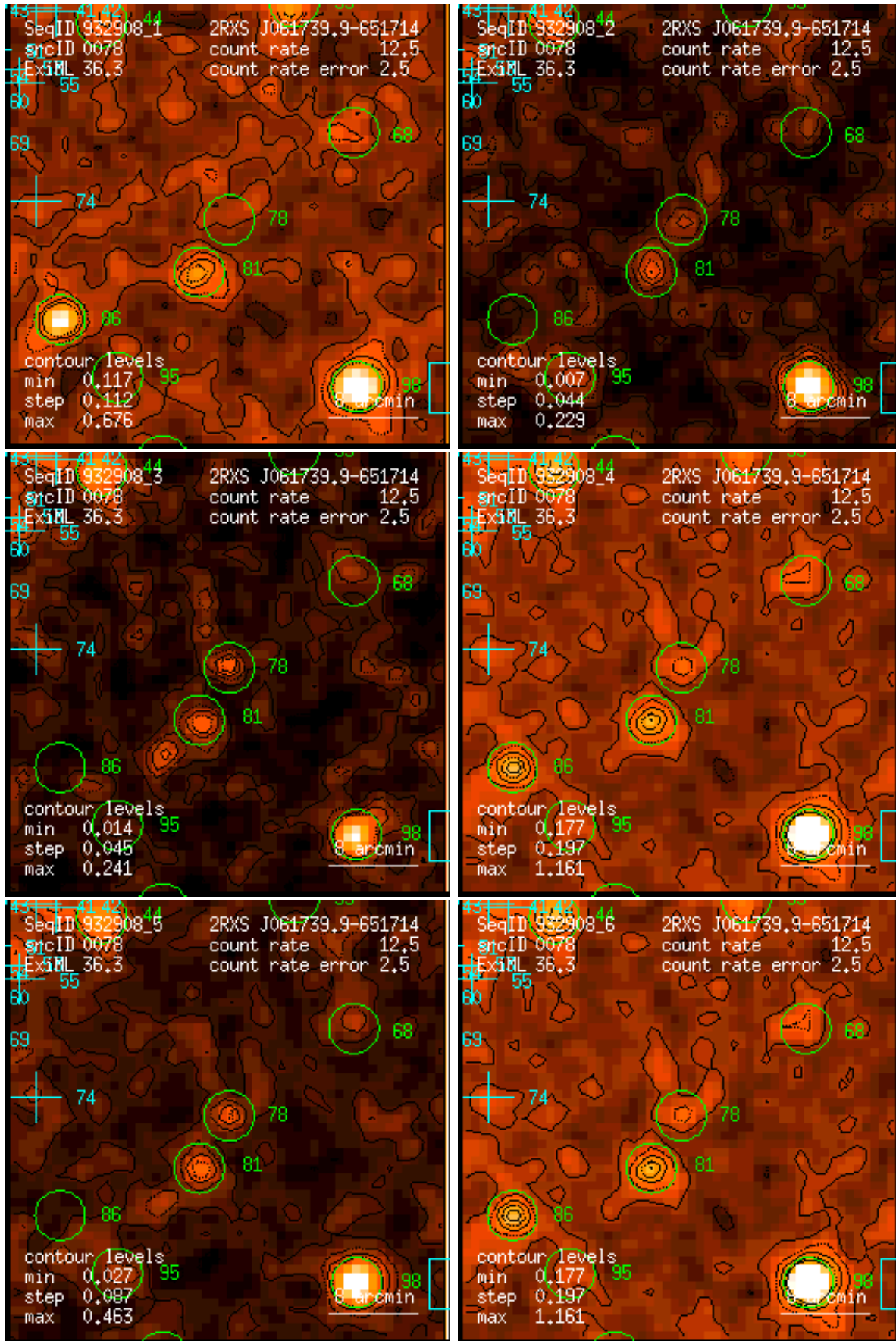
Figure 78: RASS 932908: detection 0078: band rate images, Gaussian filter: (1) PSPC channels 11 – 41, (2) 52 – 90, (3) 91 – 201, (4) 11 – 235, (5) 52 – 201, (6) 11 – 201. Broad band rates in counts/ks. Band rate contour levels in counts/ks/arcmin 2 .
