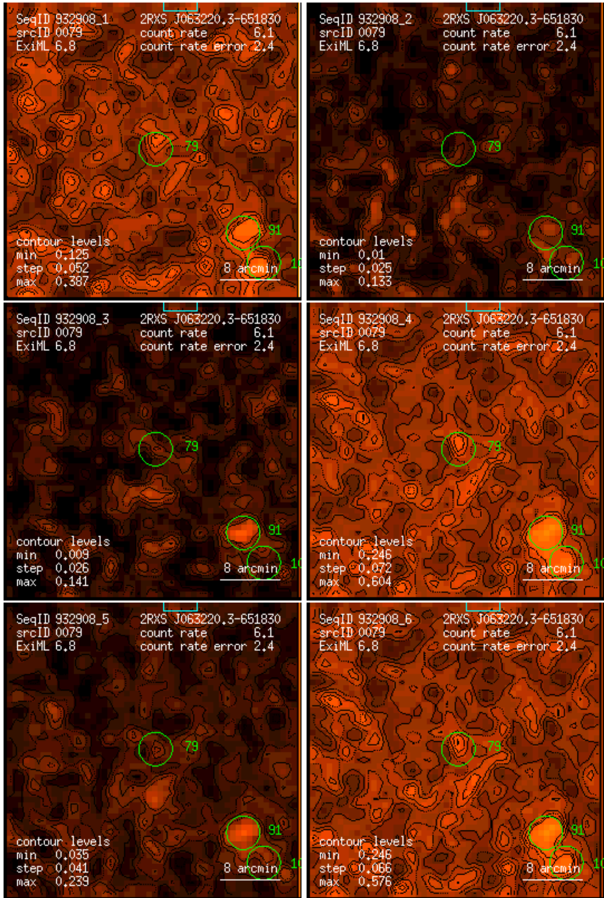
Figure 79: RASS 932908: detection 0079: band rate images, Gaussian filter: (1) PSPC channels 11 – 41, (2) 52 – 90, (3) 91 – 201, (4) 11 – 235, (5) 52 – 201, (6) 11 – 201. Broad band rates in counts/ks. Band rate contour levels in counts/ks/arcmin 2 .
