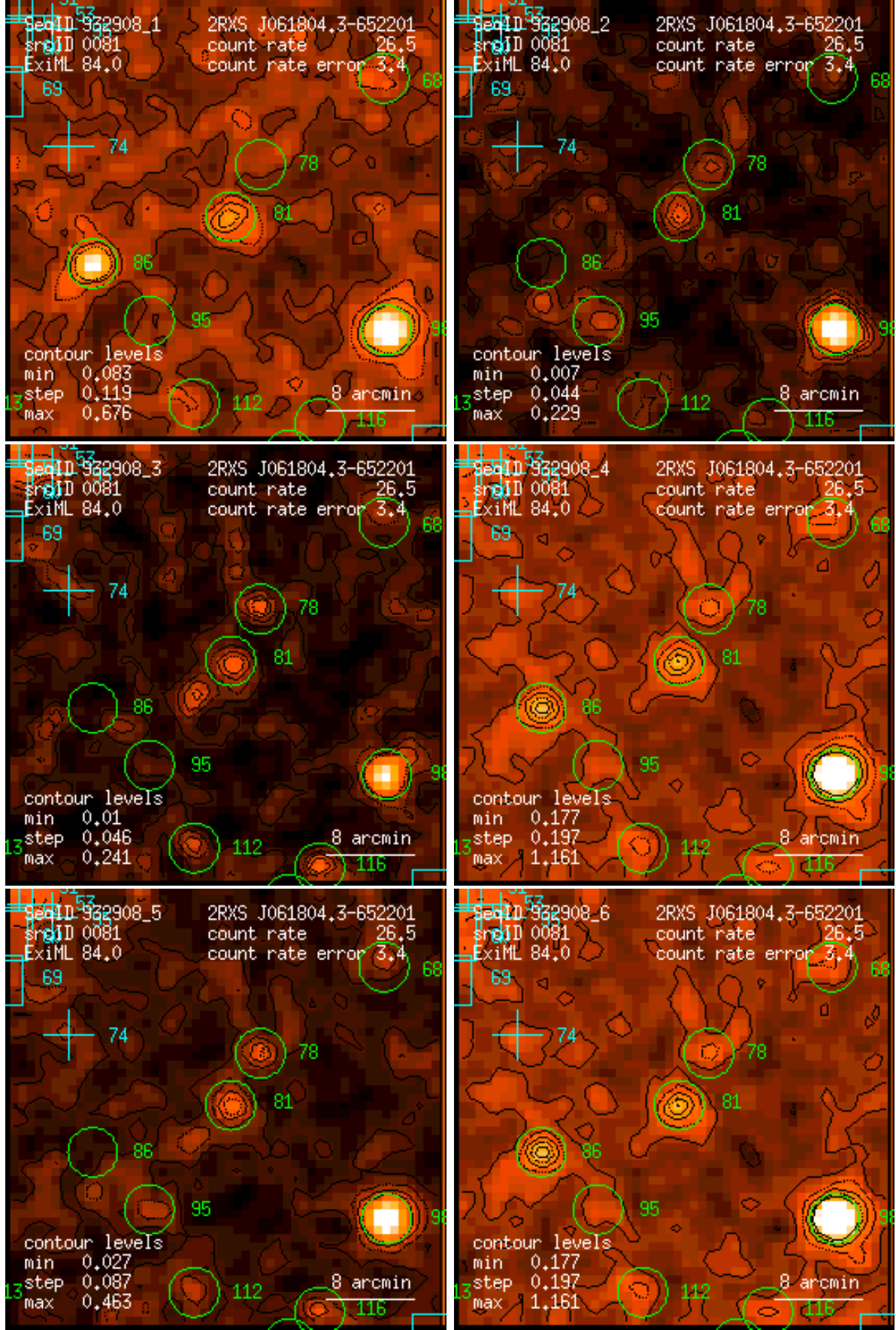
Figure 81: RASS 932908: detection 0081: band rate images, Gaussian filter: (1) PSPC channels 11 – 41, (2) 52 – 90, (3) 91 – 201, (4) 11 – 235, (5) 52 – 201, (6) 11 – 201. Broad band rates in counts/ks. Band rate contour levels in counts/ks/arcmin 2 .
