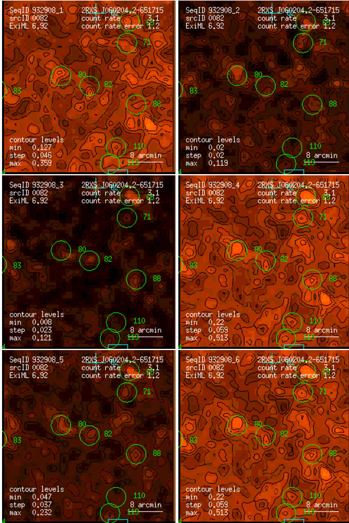
Figure 82: RASS 932908: detection 0082: band rate images, Gaussian filter: (1) PSPC channels 11 – 41, (2) 52 – 90, (3) 91 – 201, (4) 11 – 235, (5) 52 – 201, (6) 11 – 201. Broad band rates in counts/ks. Band rate contour levels in counts/ks/arcmin 2 .
