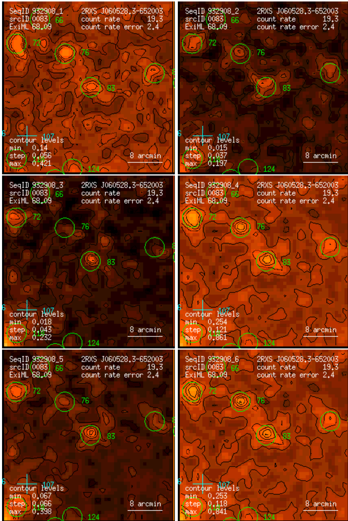
Figure 83: RASS 932908: detection 0083: band rate images, Gaussian filter: (1) PSPC channels 11 – 41, (2) 52 – 90, (3) 91 – 201, (4) 11 – 235, (5) 52 – 201, (6) 11 – 201. Broad band rates in counts/ks. Band rate contour levels in counts/ks/arcmin 2 .
