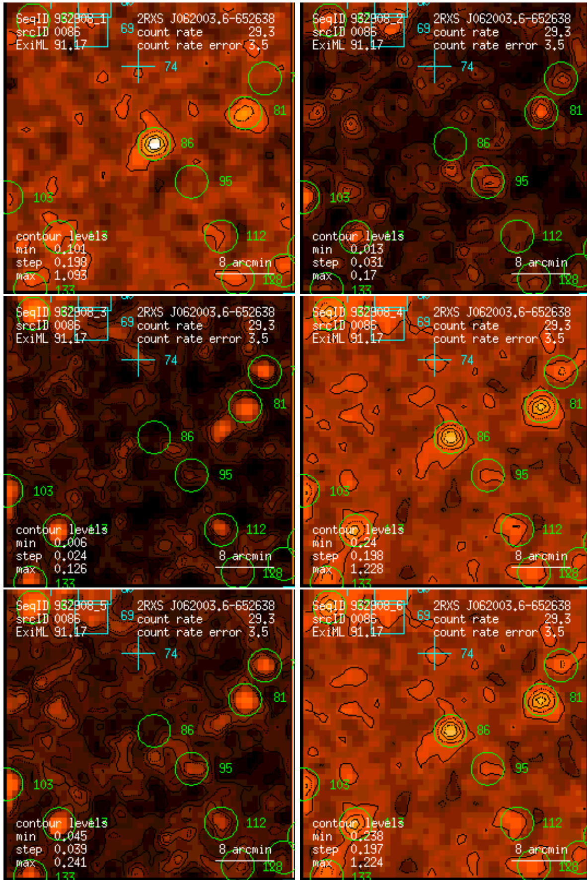
Figure 86: RASS 932908: detection 0086: band rate images, Gaussian filter: (1) PSPC channels 11 – 41, (2) 52 – 90, (3) 91 – 201, (4) 11 – 235, (5) 52 – 201, (6) 11 – 201. Broad band rates in counts/ks. Band rate contour levels in counts/ks/arcmin 2 .
