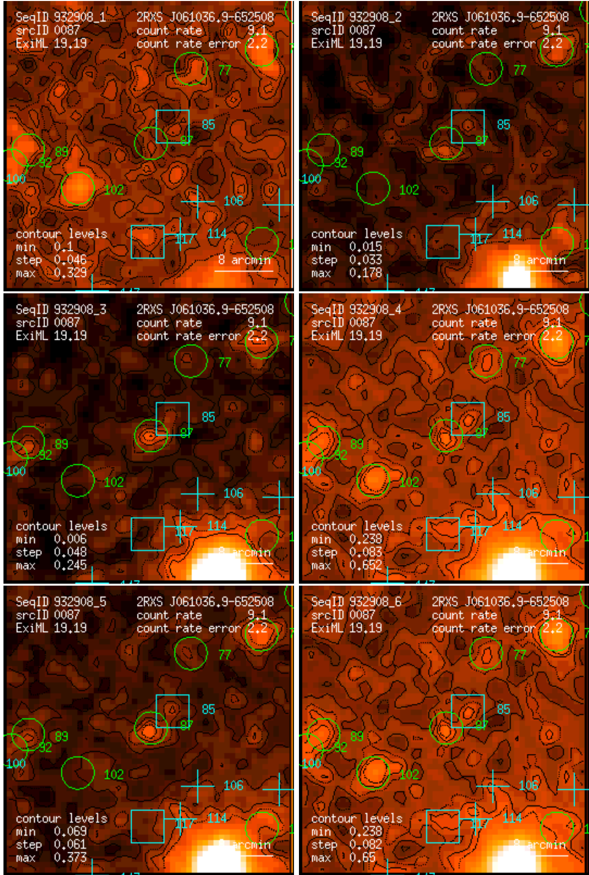
Figure 87: RASS 932908: detection 0087: band rate images, Gaussian filter: (1) PSPC channels 11 – 41, (2) 52 – 90, (3) 91 – 201, (4) 11 – 235, (5) 52 – 201, (6) 11 – 201. Broad band rates in counts/ks. Band rate contour levels in counts/ks/arcmin 2 .
