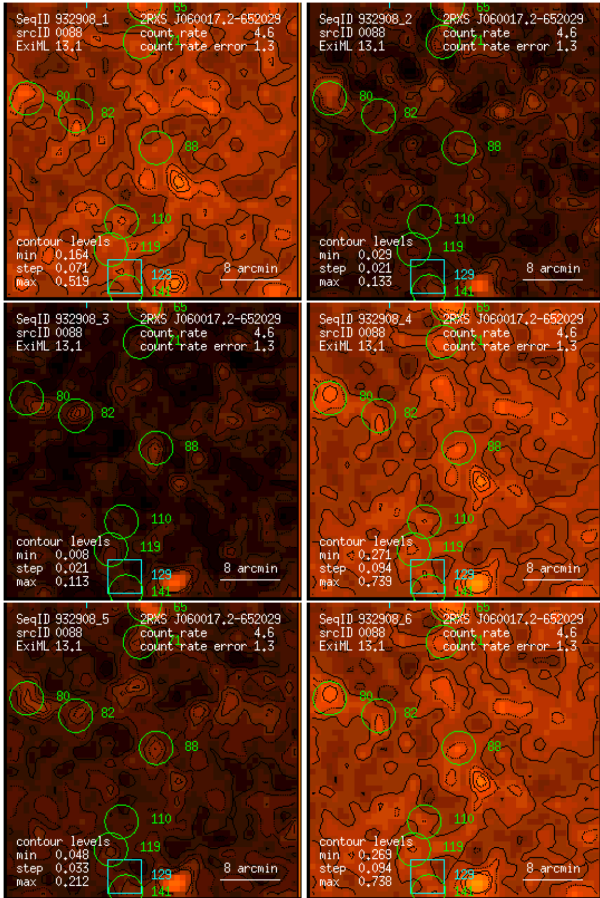
Figure 88: RASS 932908: detection 0088: band rate images, Gaussian filter: (1) PSPC channels 11 – 41, (2) 52 – 90, (3) 91 – 201, (4) 11 – 235, (5) 52 – 201, (6) 11 – 201. Broad band rates in counts/ks. Band rate contour levels in counts/ks/arcmin 2 .
