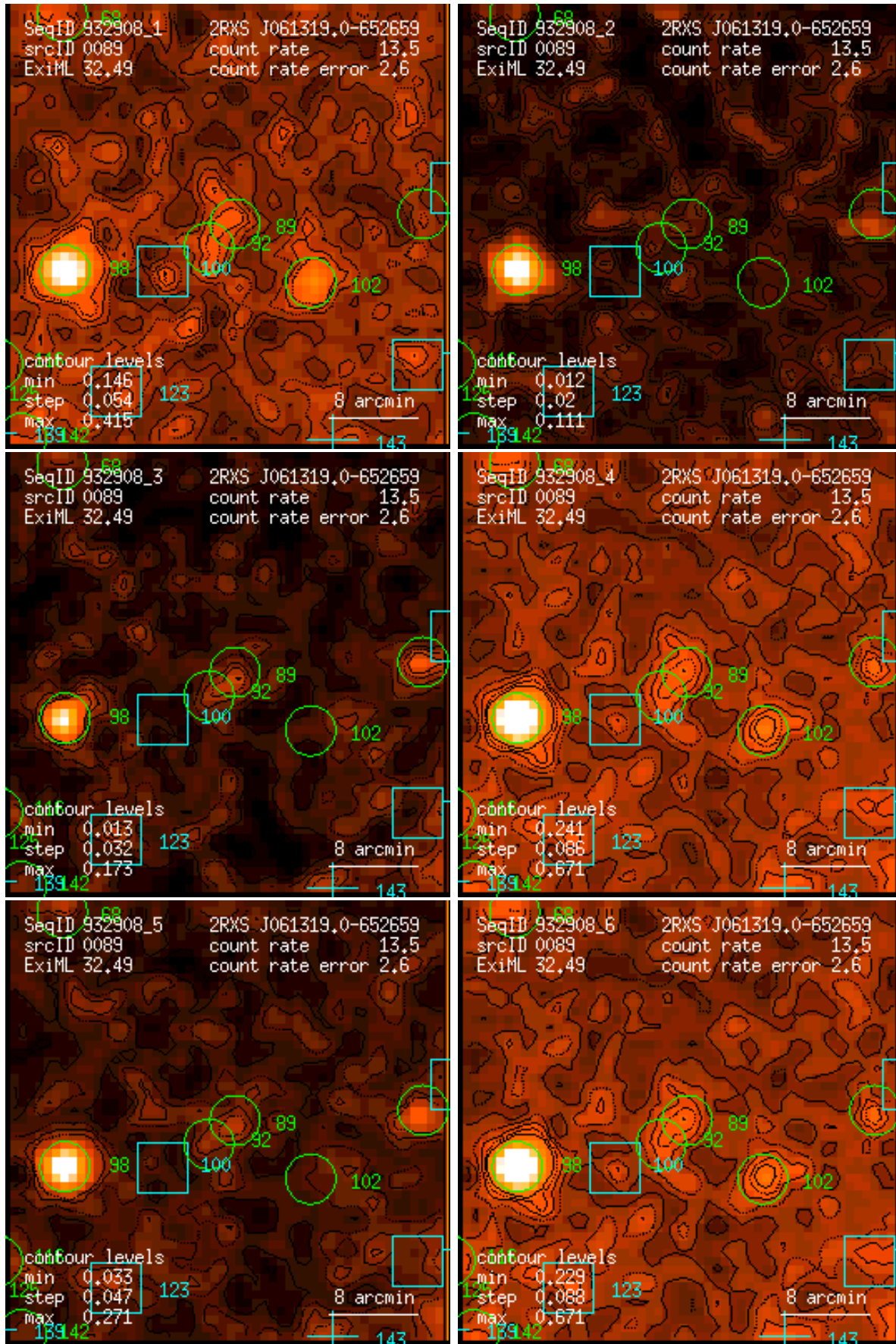
Figure 89: RASS 932908: detection 0089: band rate images, Gaussian filter: (1) PSPC channels 11 – 41, (2) 52 – 90, (3) 91 – 201, (4) 11 – 235, (5) 52 – 201, (6) 11 – 201. Broad band rates in counts/ks. Band rate contour levels in counts/ks/arcmin 2 .
