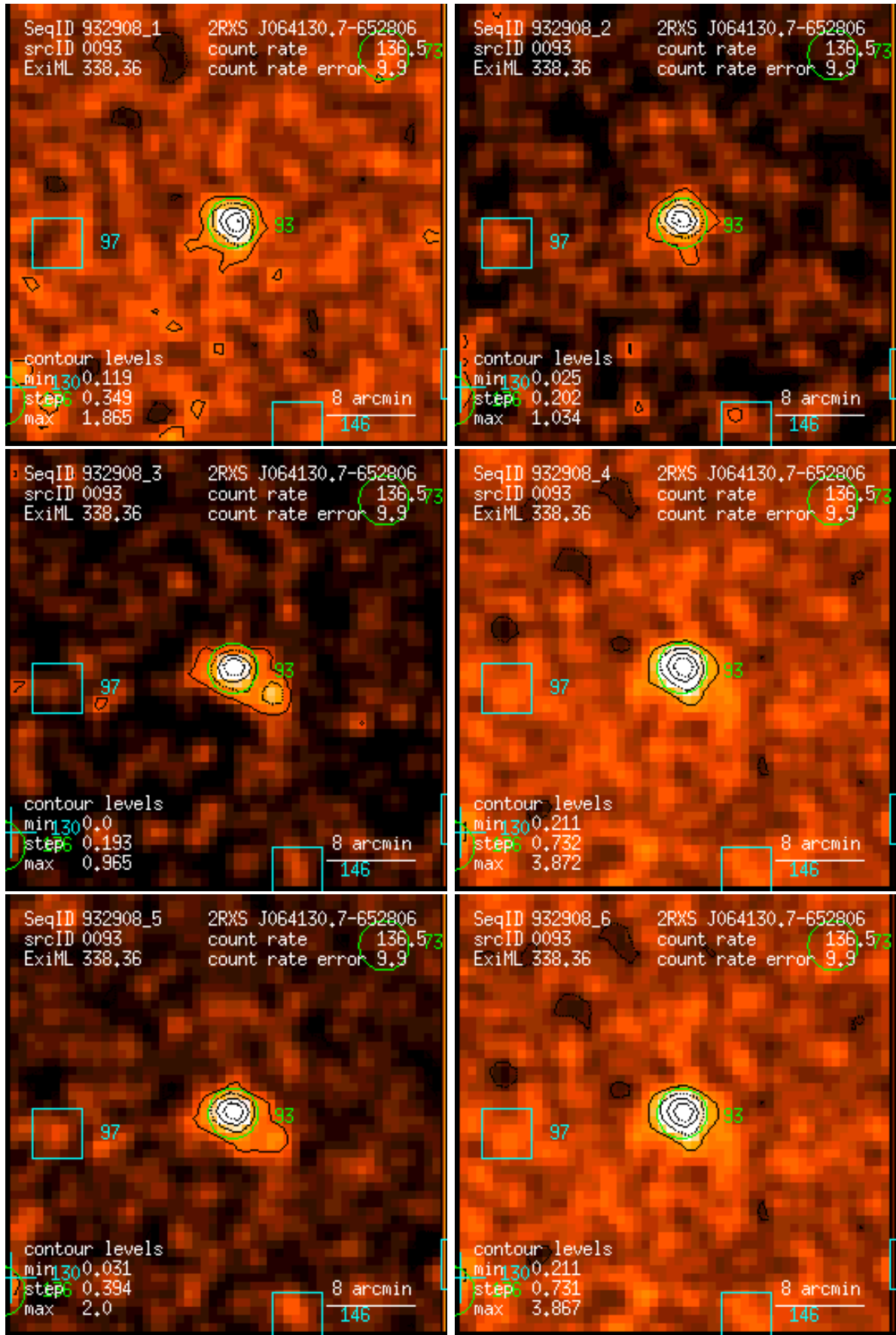
Figure 93: RASS 932908: detection 0093: band rate images, Gaussian filter: (1) PSPC channels 11 – 41, (2) 52 – 90, (3) 91 – 201, (4) 11 – 235, (5) 52 – 201, (6) 11 – 201. Broad band rates in counts/ks. Band rate contour levels in counts/ks/arcmin 2 .
